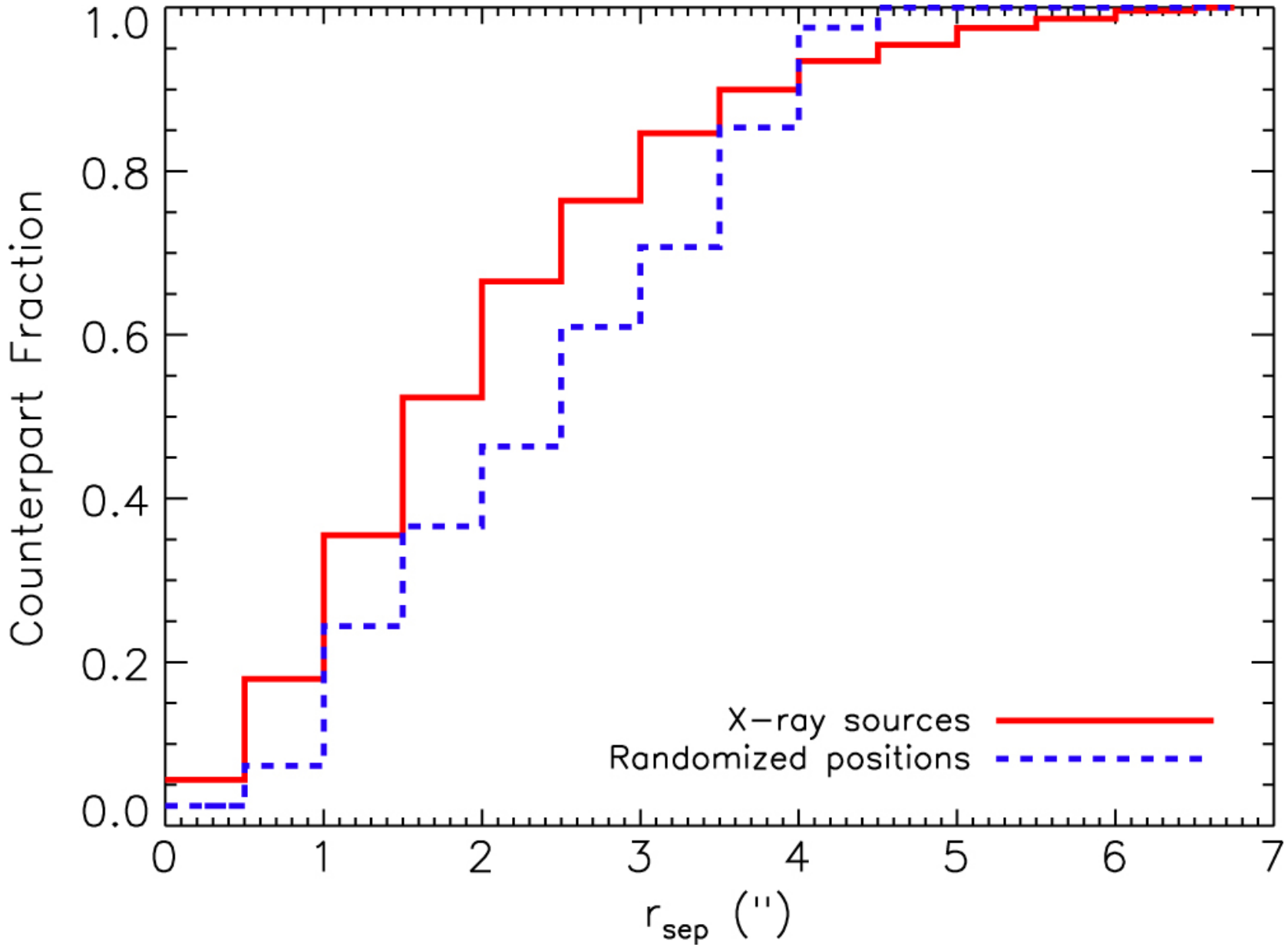
Figure 7. from THE 31 DEG2 RELEASE OF THE STRIPE 82 X-RAY SURVEY: THE POINT SOURCE CATALOG null 2016 APJ 817 172 doi:10.3847/0004-637X/817/2/172 https://dx.doi.org/10.3847/0004-637X/817/2/172 © 2016. The American Astronomical Society. All rights reserved.
