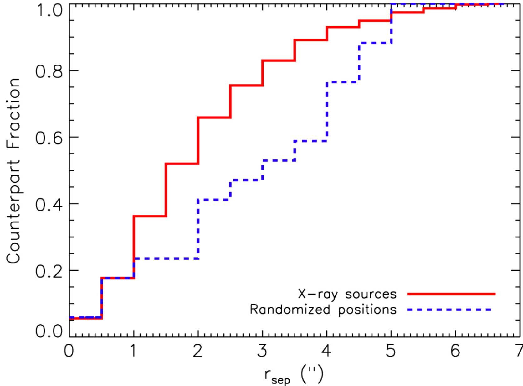
Figure 6. from THE 31 DEG2 RELEASE OF THE STRIPE 82 X-RAY SURVEY: THE POINT SOURCE CATALOG null 2016 APJ 817 172 doi:10.3847/0004-637X/817/2/172 https://dx.doi.org/10.3847/0004-637X/817/2/172 © 2016. The American Astronomical Society. All rights reserved.
