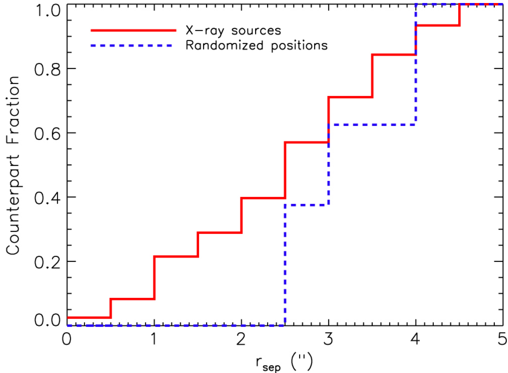
Figure 10. from THE 31 DEG2 RELEASE OF THE STRIPE 82 X-RAY SURVEY: THE POINT SOURCE CATALOG null 2016 APJ 817 172 doi:10.3847/0004-637X/817/2/172 https://dx.doi.org/10.3847/0004-637X/817/2/172 © 2016. The American Astronomical Society. All rights reserved.
