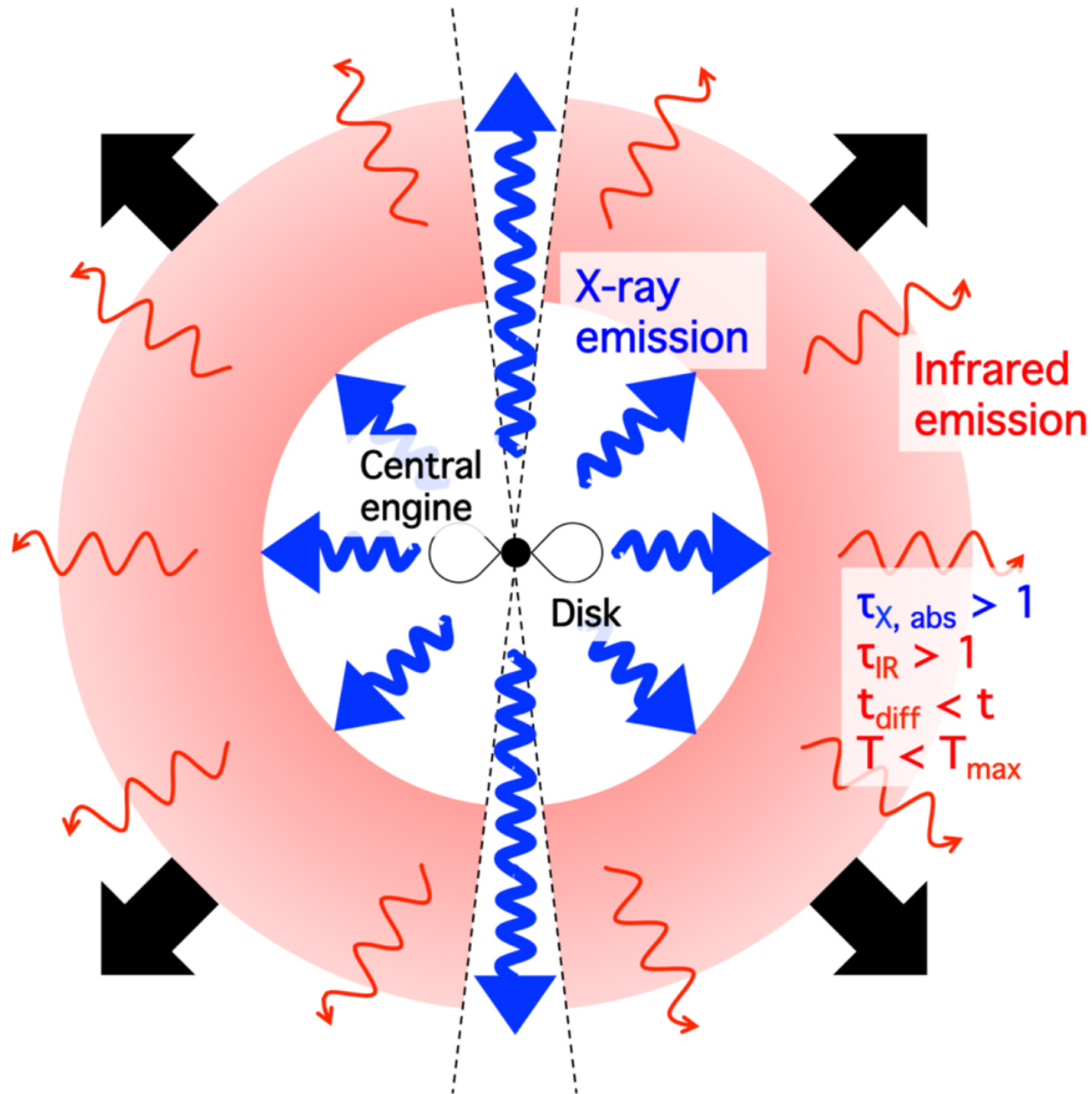
Figure 2. from X-RAY-POWERED MACRONOVAE null 2016 APJ 818 104 doi:10.3847/0004-637X/818/2/104 https://dx.doi.org/10.3847/0004-637X/818/2/104 © 2016. The American Astronomical Society. All rights reserved.
