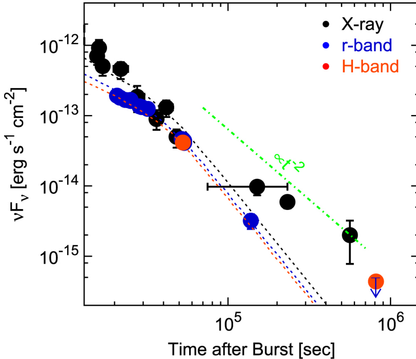
Figure 1. from X-RAY-POWERED MACRONOVAE null 2016 APJ 818 104 doi:10.3847/0004-637X/818/2/104 https://dx.doi.org/10.3847/0004-637X/818/2/104 © 2016. The American Astronomical Society. All rights reserved.
