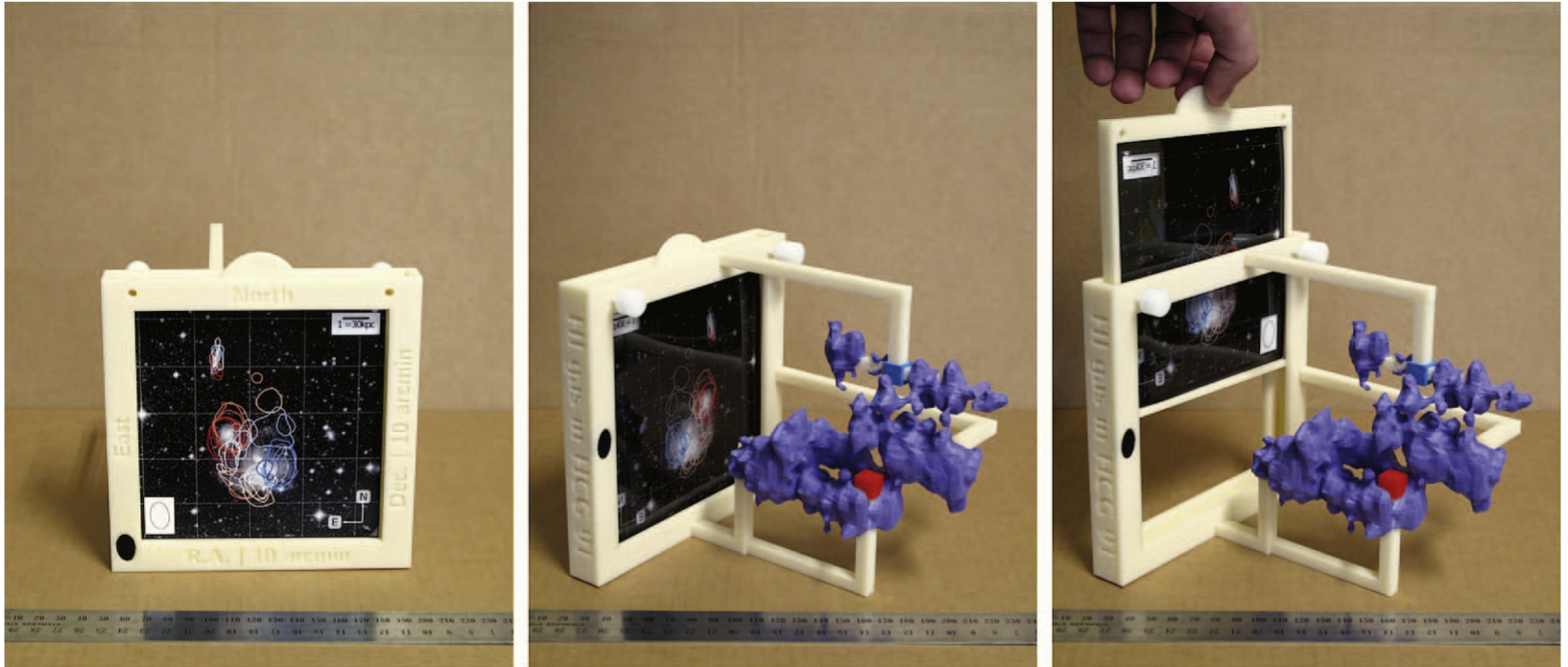
Figure 4. from ADVANCED DATA VISUALIZATION IN ASTROPHYSICS: THE X3D PATHWAY null 2016 APJ 818 115 doi:10.3847/0004-637X/818/2/115 https://dx.doi.org/10.3847/0004-637X/818/2/115 © 2016. The American Astronomical Society. All rights reserved.
