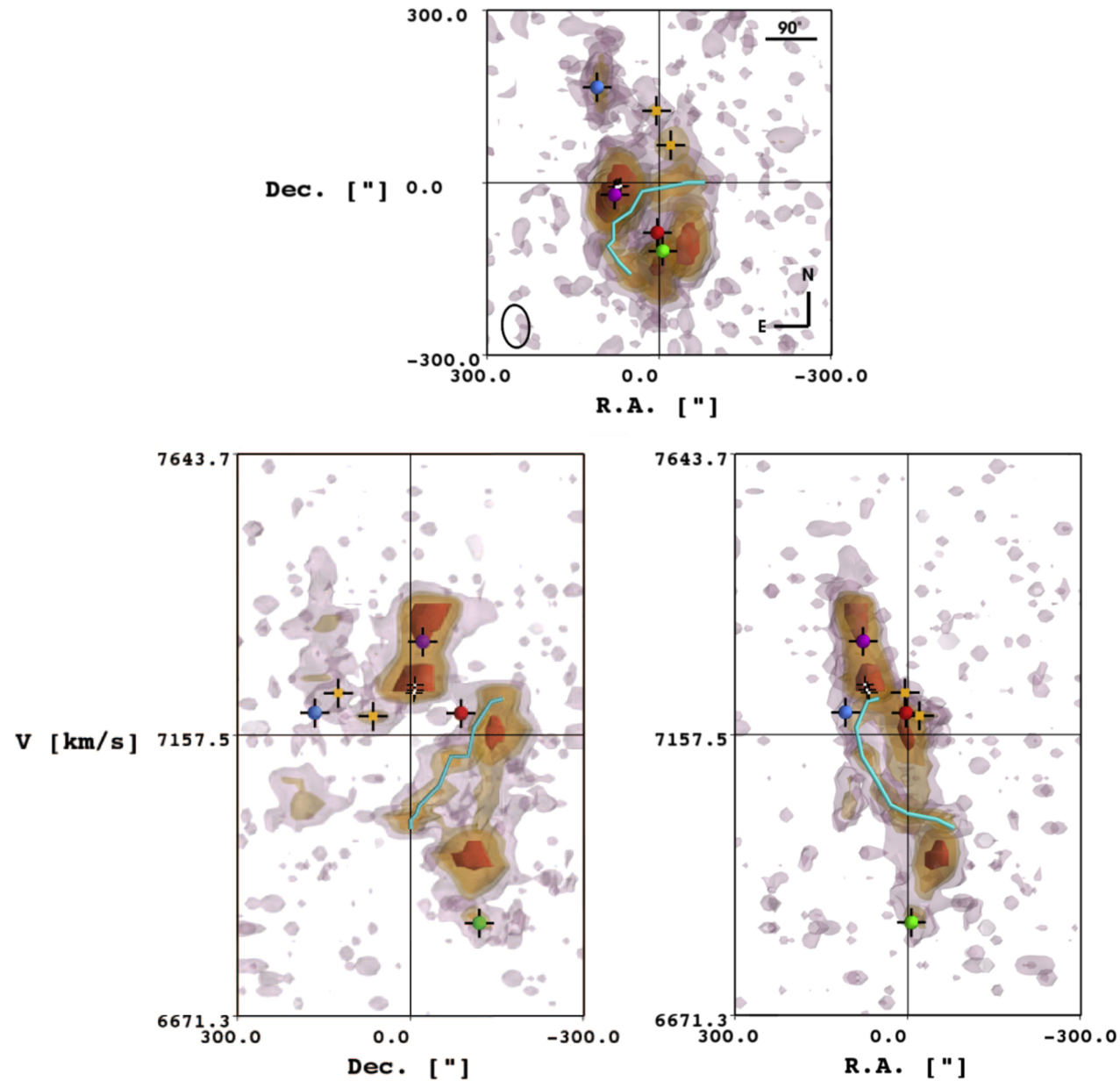
Figure 3. from ADVANCED DATA VISUALIZATION IN ASTROPHYSICS: THE X3D PATHWAY null 2016 APJ 818 115 doi:10.3847/0004-637X/818/2/115 https://dx.doi.org/10.3847/0004-637X/818/2/115 © 2016. The American Astronomical Society. All rights reserved.
