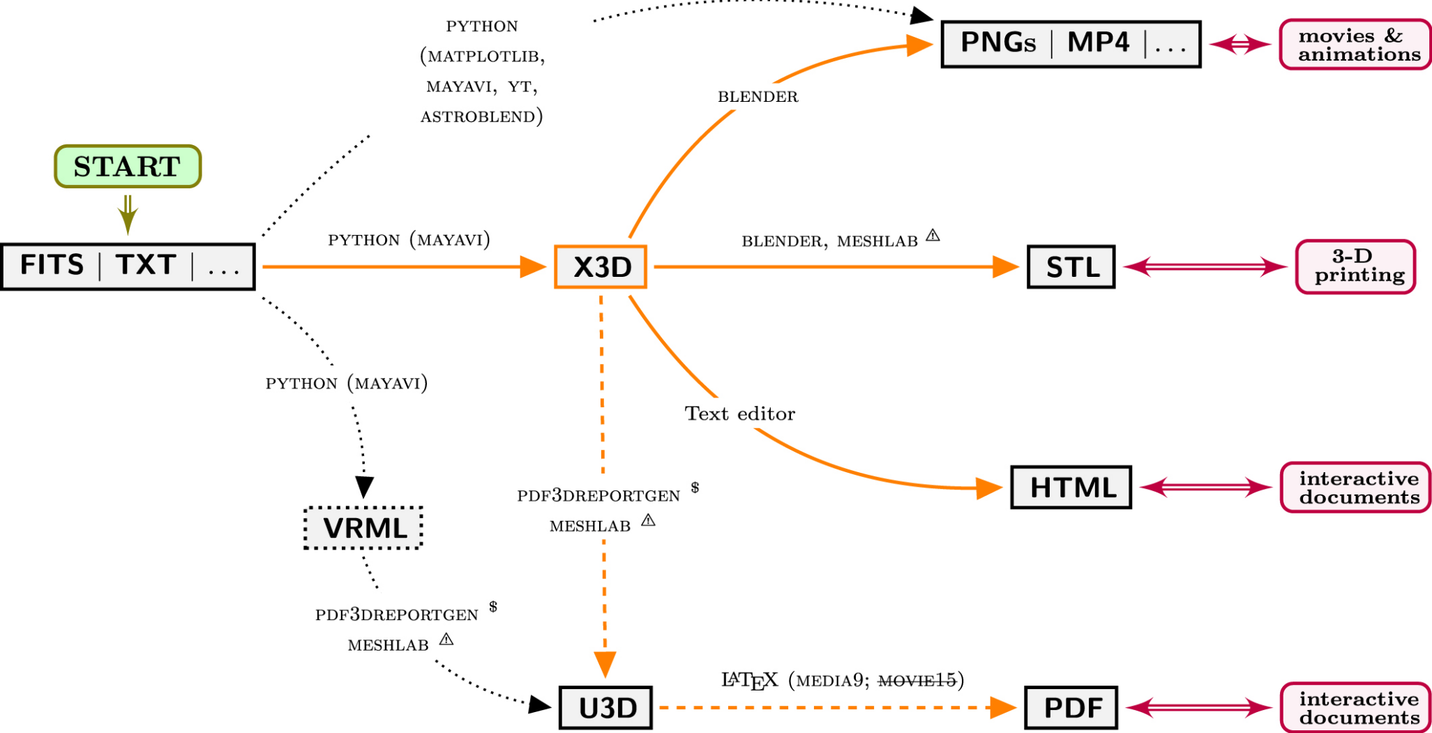
Figure 1. from ADVANCED DATA VISUALIZATION IN ASTROPHYSICS: THE X3D PATHWAY null 2016 APJ 818 115 doi:10.3847/0004-637X/818/2/115 https://dx.doi.org/10.3847/0004-637X/818/2/115 © 2016. The American Astronomical Society. All rights reserved.
