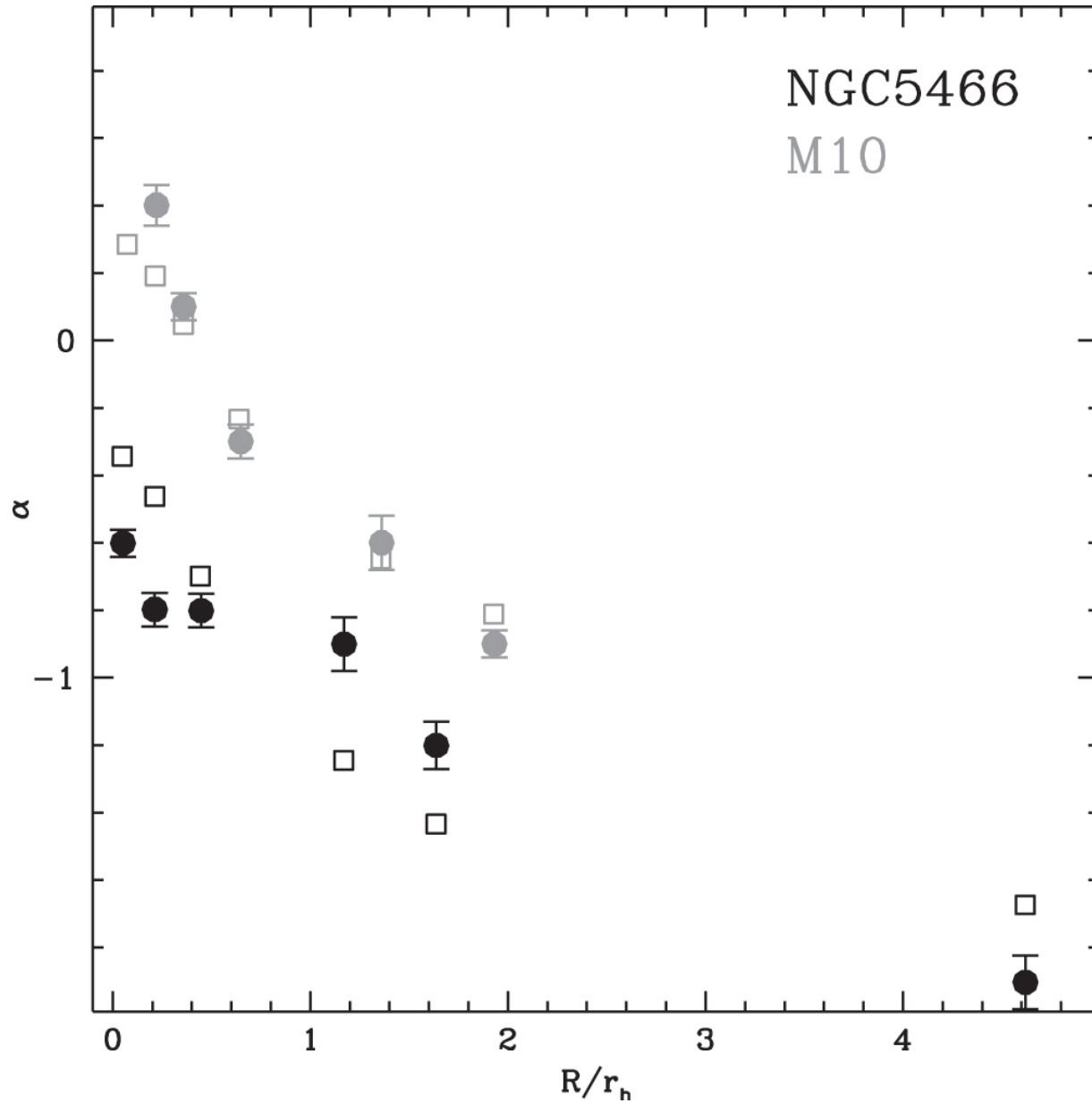
Figure 6. from DEEP MULTI-TELESCOPE PHOTOMETRY OF NGC 5466. II. THE RADIAL BEHAVIOR OF THE MASS FUNCTION SLOPE null 2015 APJ 814 144 doi:10.1088/0004-637X/814/2/144 https://dx.doi.org/10.1088/0004-637X/814/2/144 © 2015. The American Astronomical Society. All rights reserved.
