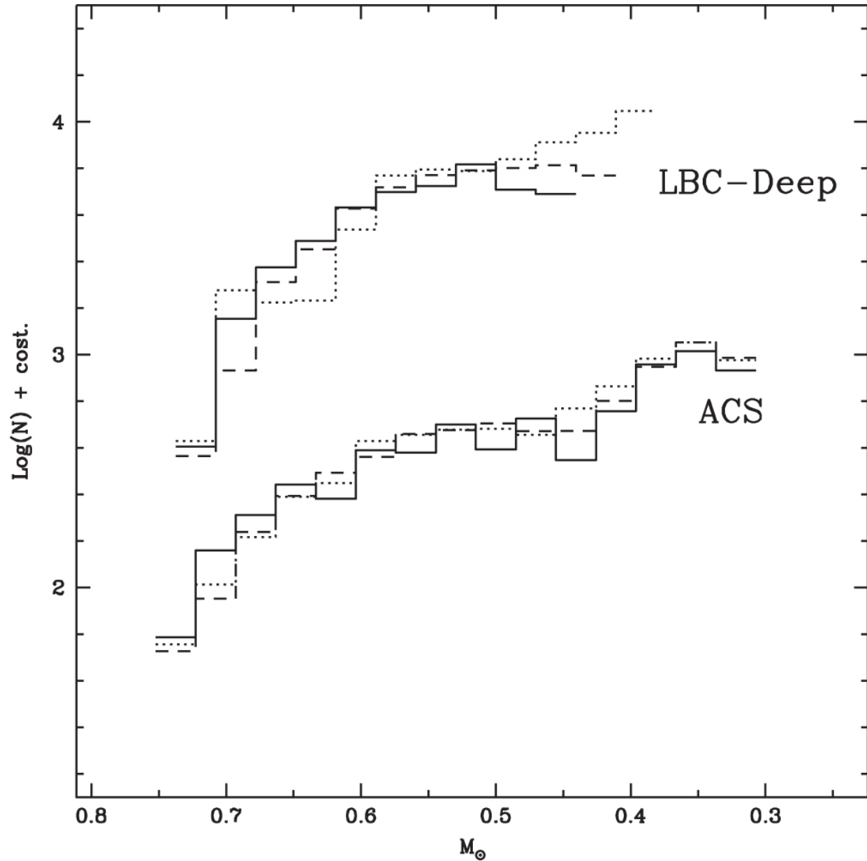
Figure 5. from DEEP MULTI-TELESCOPE PHOTOMETRY OF NGC 5466. II. THE RADIAL BEHAVIOR OF THE MASS FUNCTION SLOPE null 2015 APJ 814 144 doi:10.1088/0004-637X/814/2/144 https://dx.doi.org/10.1088/0004-637X/814/2/144 © 2015. The American Astronomical Society. All rights reserved.
