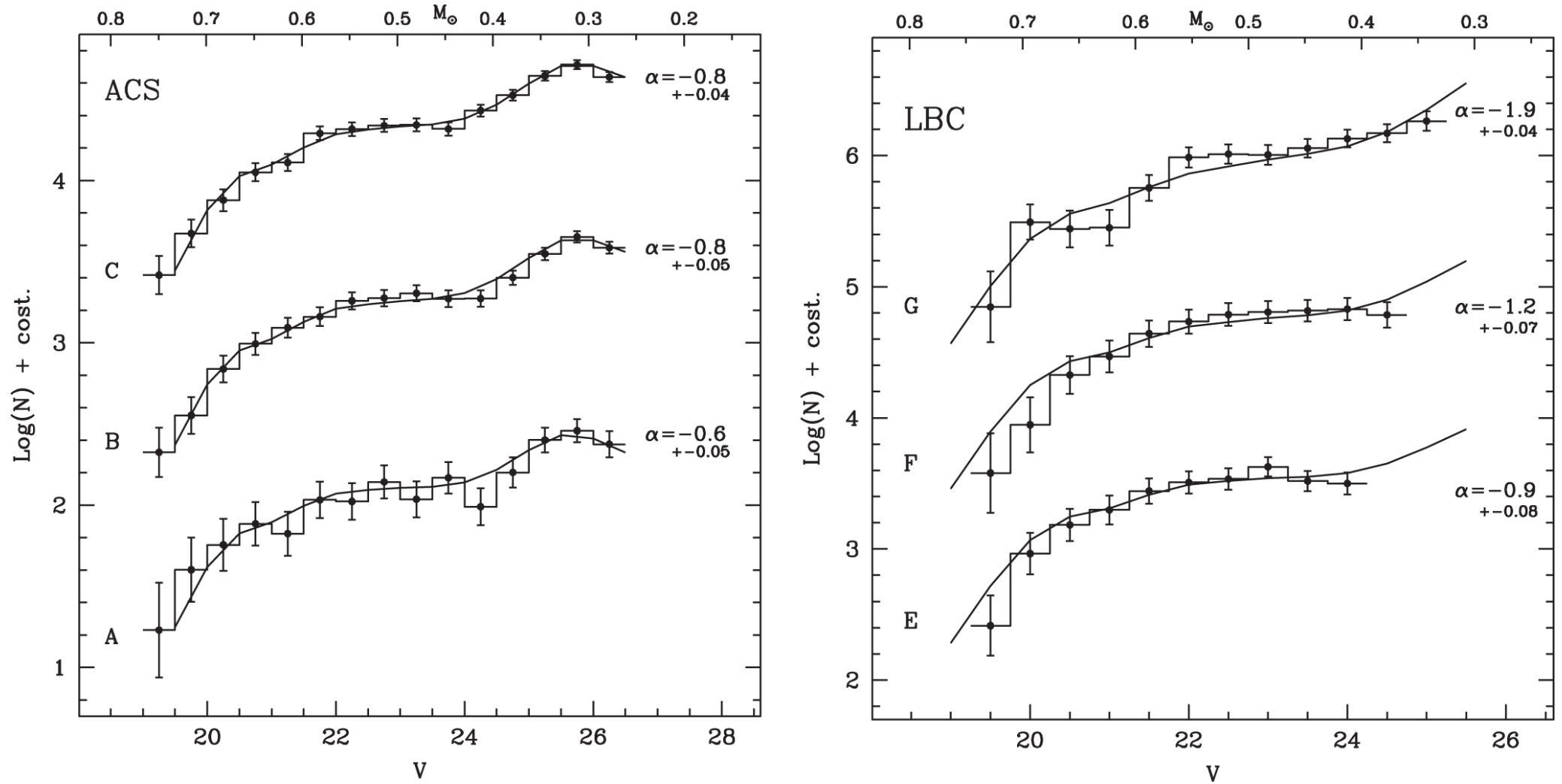
Figure 4. from DEEP MULTI-TELESCOPE PHOTOMETRY OF NGC 5466. II. THE RADIAL BEHAVIOR OF THE MASS FUNCTION SLOPE null 2015 APJ 814 144 doi:10.1088/0004-637X/814/2/144 https://dx.doi.org/10.1088/0004-637X/814/2/144 © 2015. The American Astronomical Society. All rights reserved.
