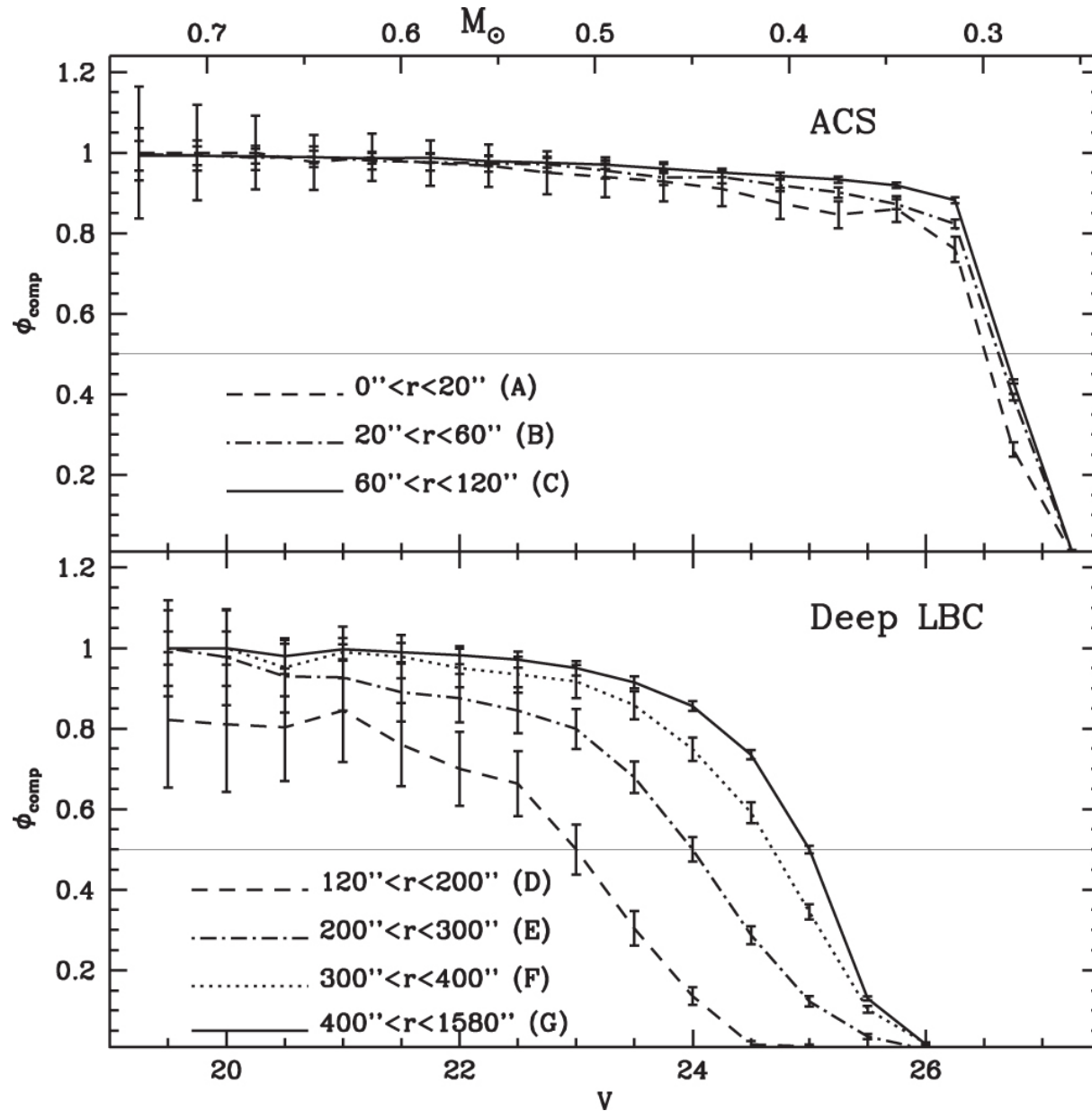
Figure 3. from DEEP MULTI-TELESCOPE PHOTOMETRY OF NGC 5466. II. THE RADIAL BEHAVIOR OF THE MASS FUNCTION SLOPE null 2015 APJ 814 144 doi:10.1088/0004-637X/814/2/144 https://dx.doi.org/10.1088/0004-637X/814/2/144 © 2015. The American Astronomical Society. All rights reserved.
