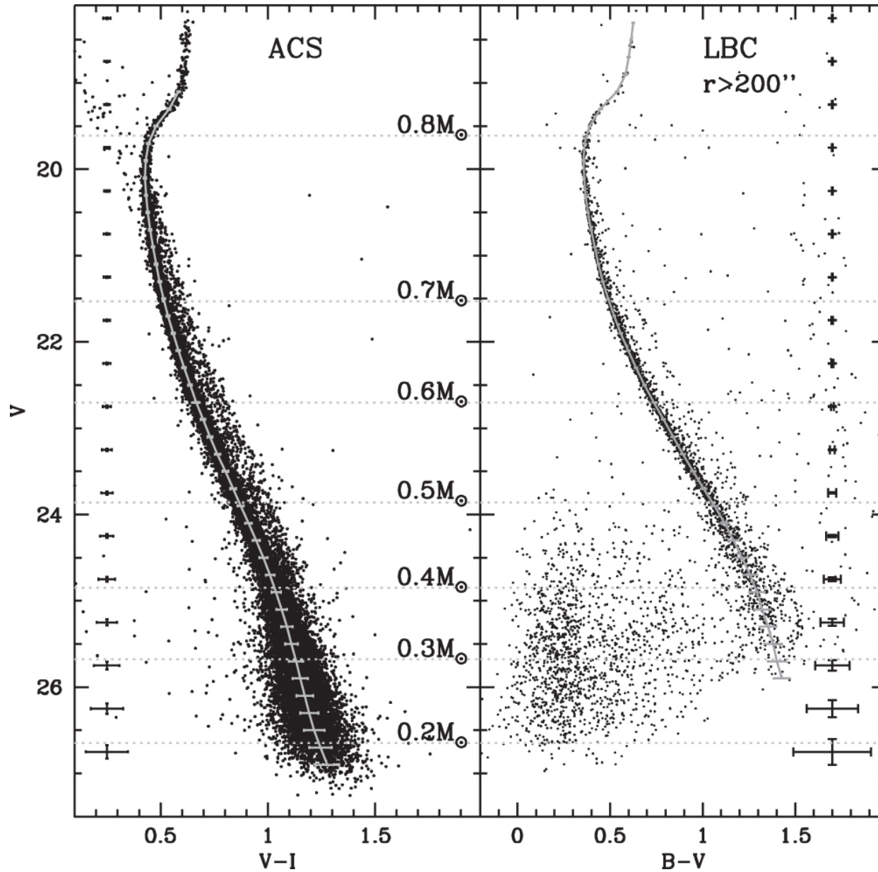
Figure 2. from DEEP MULTI-TELESCOPE PHOTOMETRY OF NGC 5466. II. THE RADIAL BEHAVIOR OF THE MASS FUNCTION SLOPE null 2015 APJ 814 144 doi:10.1088/0004-637X/814/2/144 https://dx.doi.org/10.1088/0004-637X/814/2/144 © 2015. The American Astronomical Society. All rights reserved.
