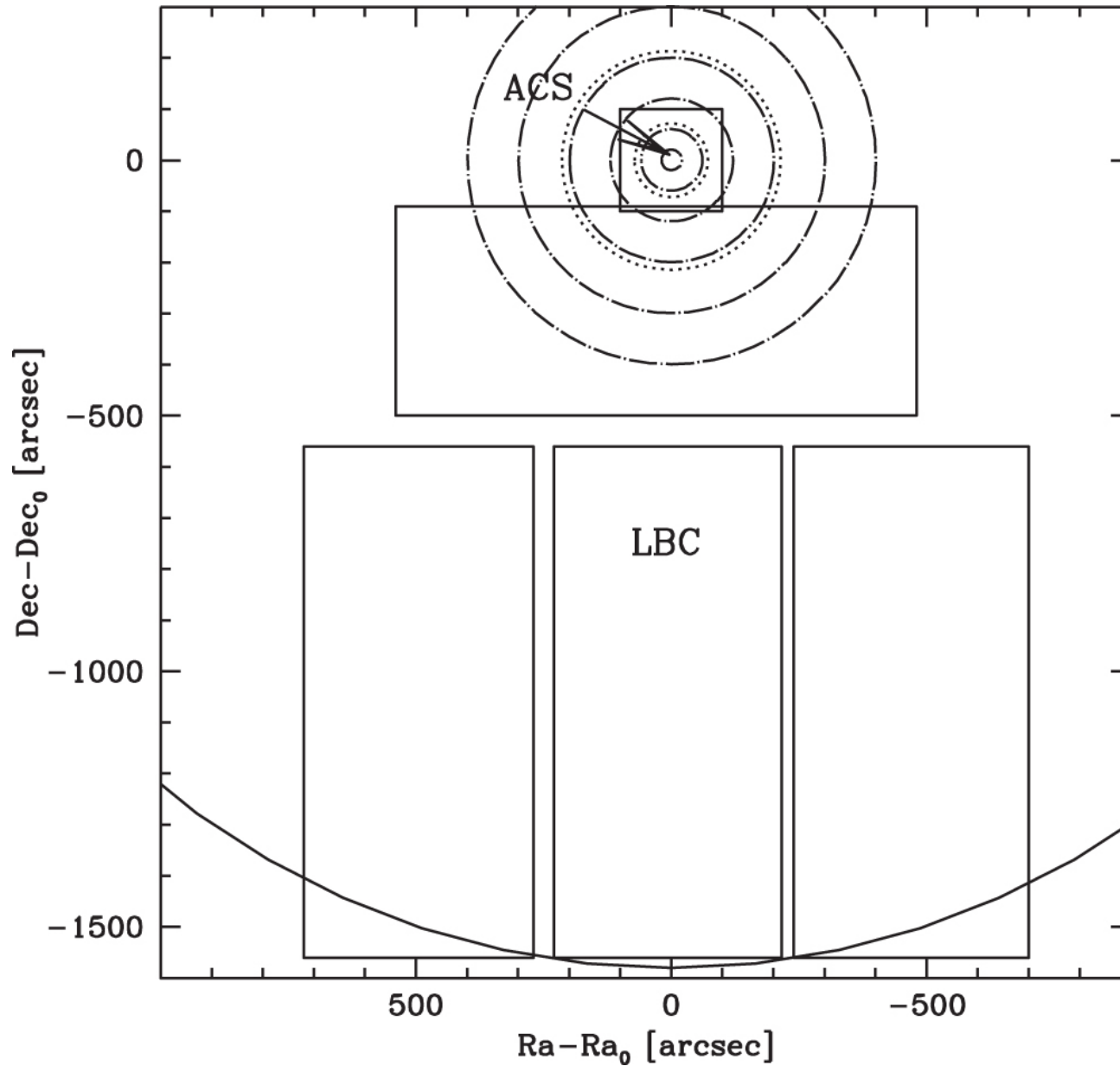
Figure 1. from DEEP MULTI-TELESCOPE PHOTOMETRY OF NGC 5466. II. THE RADIAL BEHAVIOR OF THE MASS FUNCTION SLOPE null 2015 APJ 814 144 doi:10.1088/0004-637X/814/2/144 https://dx.doi.org/10.1088/0004-637X/814/2/144 © 2015. The American Astronomical Society. All rights reserved.
