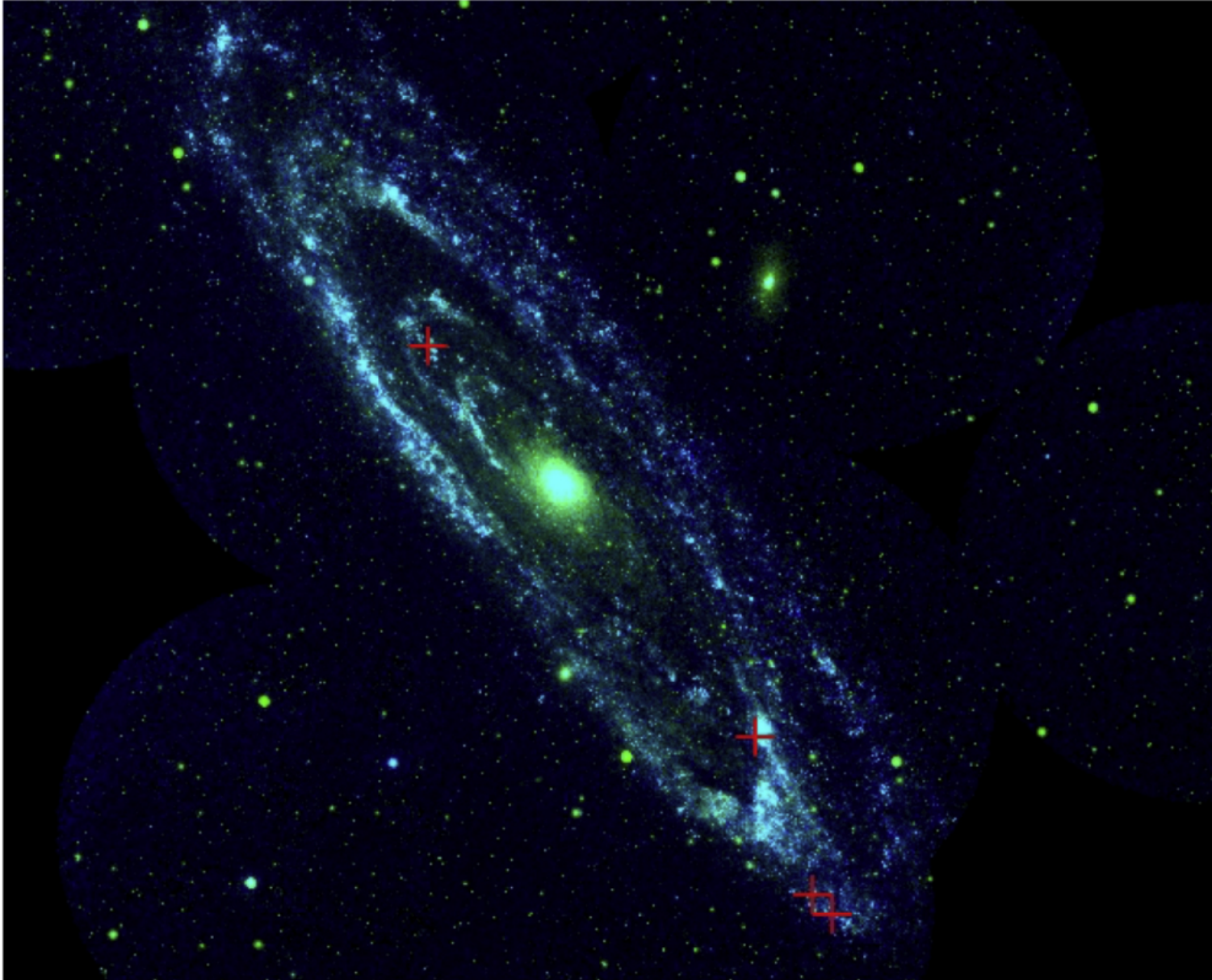
Figure 1. from NEW ULTRAVIOLET EXTINCTION CURVES FOR INTERSTELLAR DUST IN M31 null 2015 APJ 815 14 doi:10.1088/0004-637X/815/1/14 https://dx.doi.org/10.1088/0004-637X/815/1/14 © 2015. The American Astronomical Society. All rights reserved.
