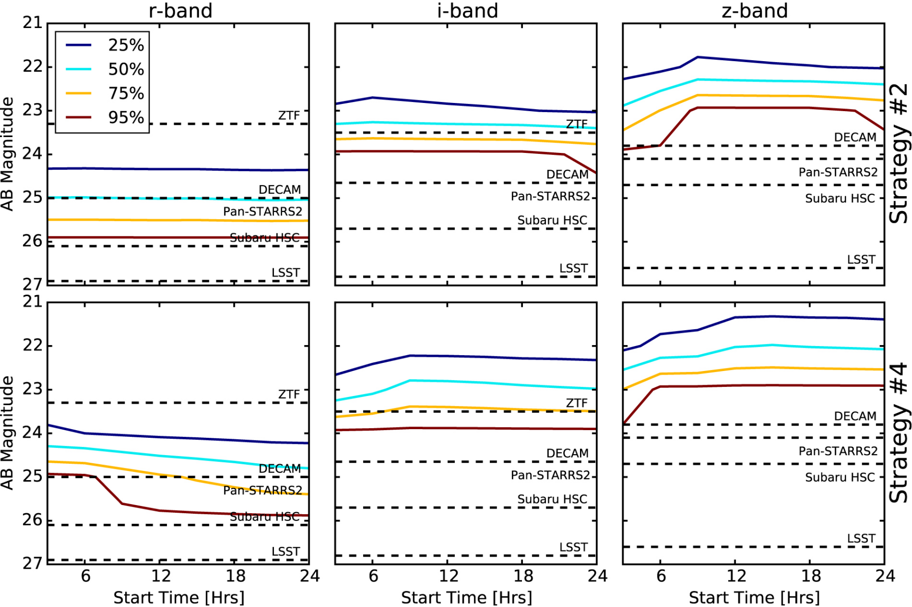
Figure 18. from A COMPREHENSIVE STUDY OF DETECTABILITY AND CONTAMINATION IN DEEP RAPID OPTICAL SEARCHES FOR GRAVITATIONAL WAVE COUNTERPARTS null 2015 APJ 814 25 doi:10.1088/0004-637X/814/1/25 https://dx.doi.org/10.1088/0004-637X/814/1/25 © 2015. The American Astronomical Society. All rights reserved.
