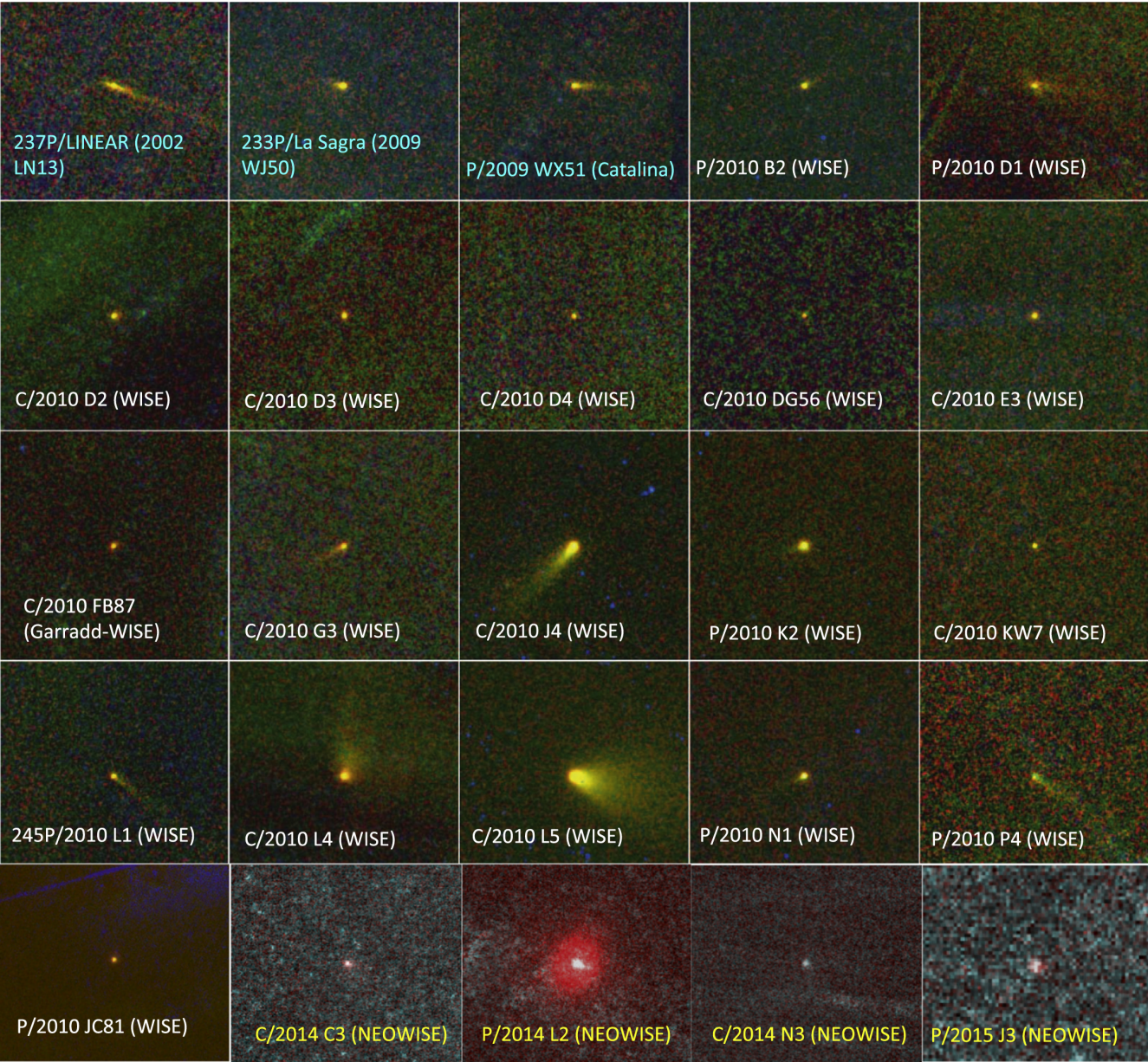
Figure 1. from THE NEOWISE-DISCOVERED COMET POPULATION AND THE CO + CO2 PRODUCTION RATES null 2015 APJ 814 85 doi:10.1088/0004-637X/814/2/85 https://dx.doi.org/10.1088/0004-637X/814/2/85 © 2015. The American Astronomical Society. All rights reserved.
