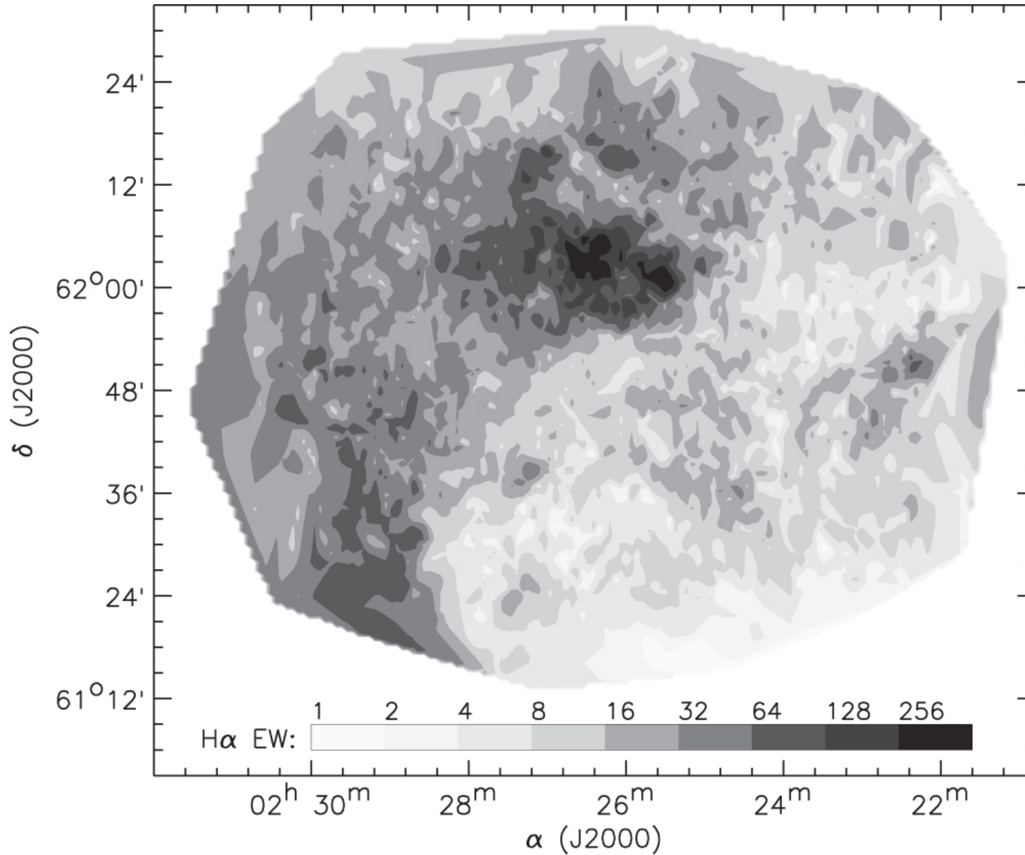
Figure 6. from THE O- AND B-TYPE STELLAR POPULATION IN W3: BEYOND THE HIGH-DENSITY LAYER null 2015 APJ 813 42 doi:10.1088/0004-637X/813/1/42 https://dx.doi.org/10.1088/0004-637X/813/1/42 © 2015. The American Astronomical Society. All rights reserved.
