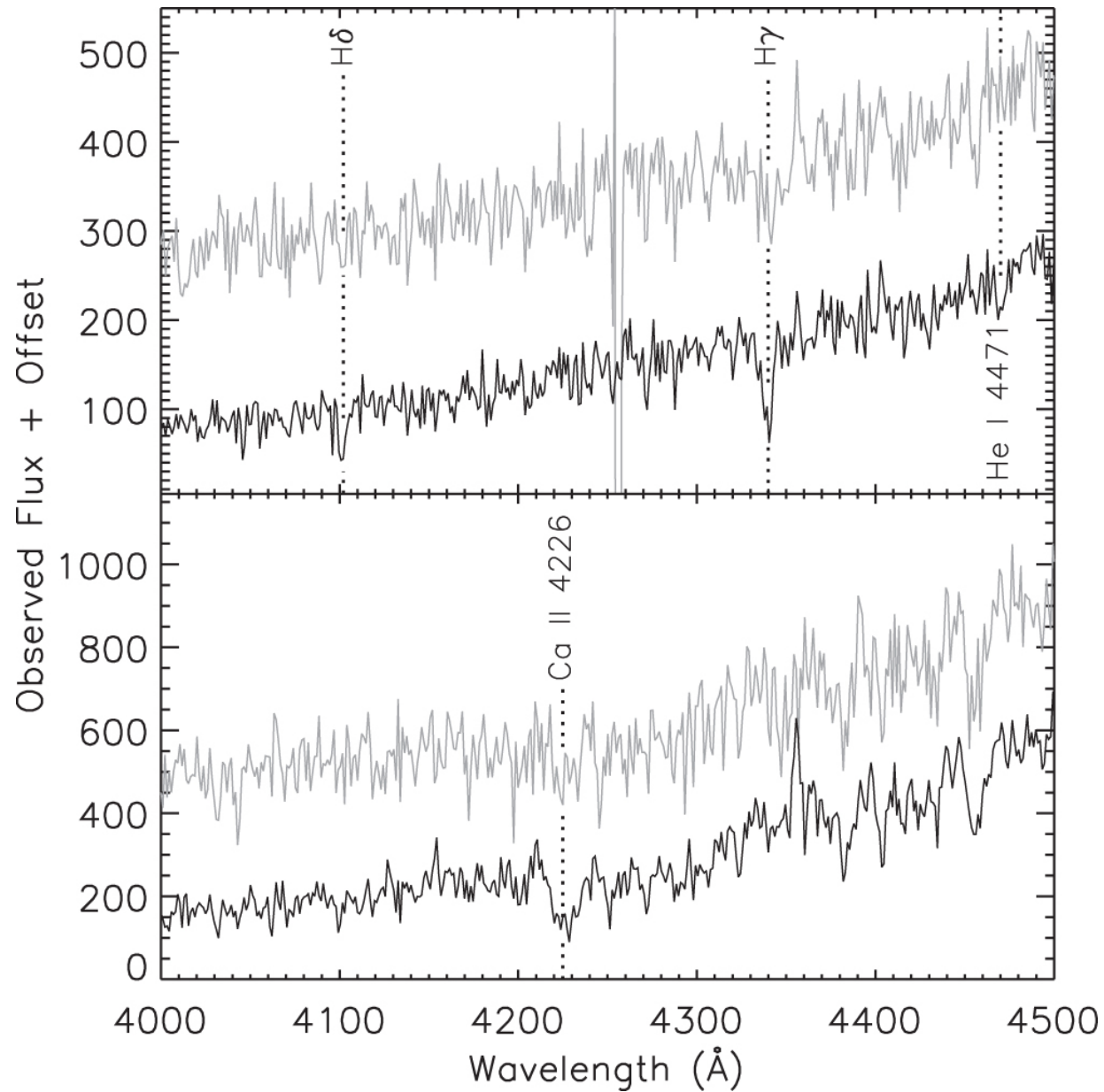
Figure 5. from THE O- AND B-TYPE STELLAR POPULATION IN W3: BEYOND THE HIGH-DENSITY LAYER null 2015 APJ 813 42 doi:10.1088/0004-637X/813/1/42 https://dx.doi.org/10.1088/0004-637X/813/1/42 © 2015. The American Astronomical Society. All rights reserved.
