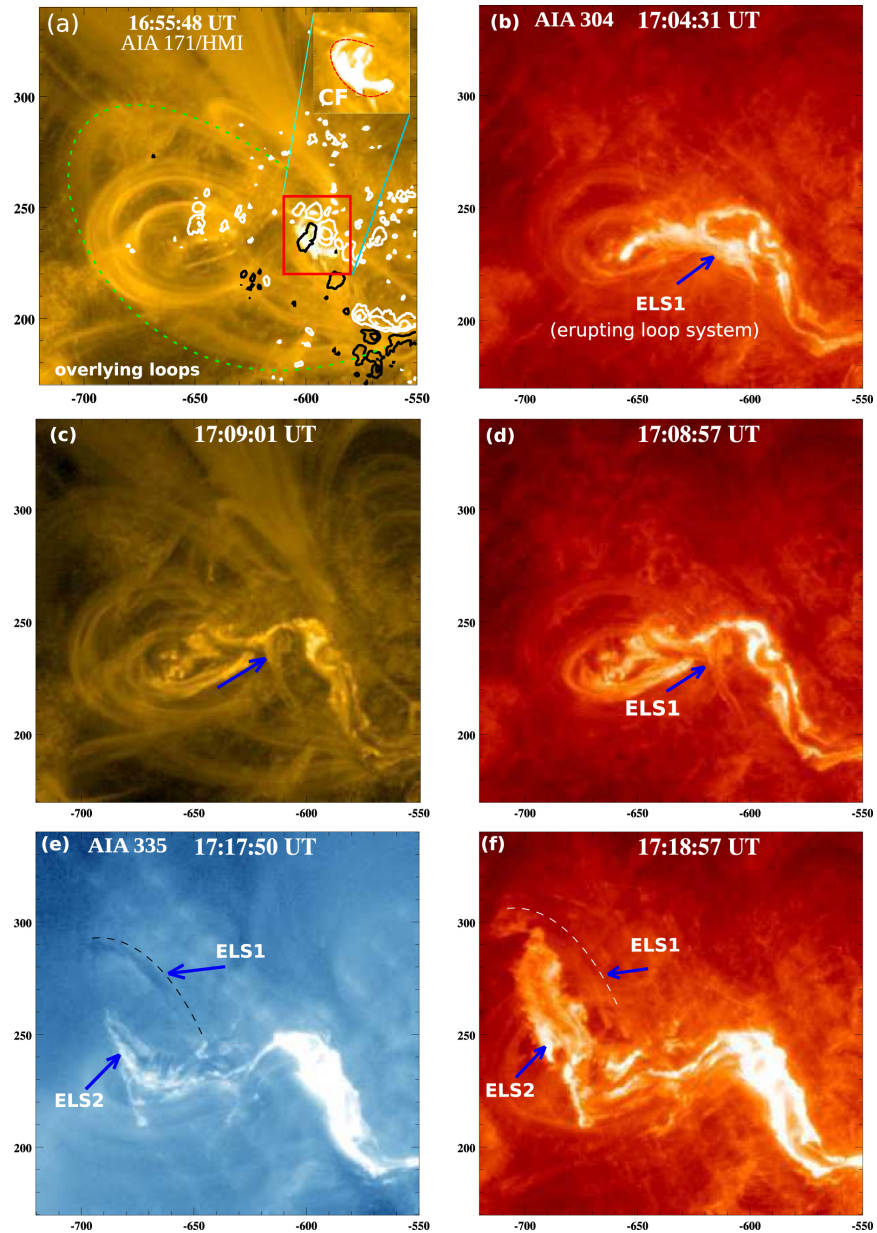
Figure 9. from MULTIWAVELENGTH OBSERVATIONS OF A SLOW-RISE, MULTISTEP X1.6 FLARE AND THE ASSOCIATED ERUPTION null 2015 APJ 812 172 doi:10.1088/0004-637X/812/2/172 https://dx.doi.org/10.1088/0004-637X/812/2/172 © 2015. The American Astronomical Society. All rights reserved.
