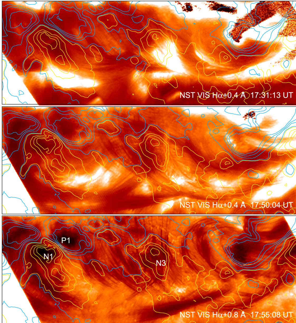
Figure 8. from MULTIWAVELENGTH OBSERVATIONS OF A SLOW-RISE, MULTISTEP X1.6 FLARE AND THE ASSOCIATED ERUPTION null 2015 APJ 812 172 doi:10.1088/0004-637X/812/2/172 https://dx.doi.org/10.1088/0004-637X/812/2/172 © 2015. The American Astronomical Society. All rights reserved.
