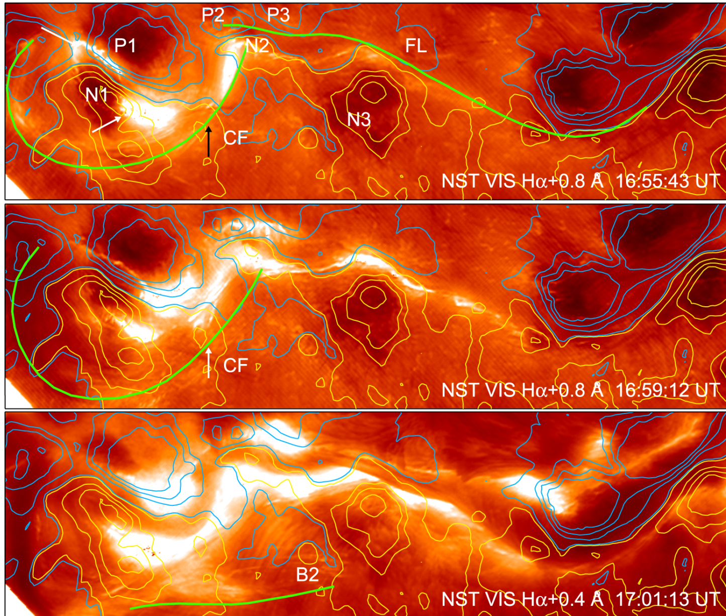
Figure 7. from MULTIWAVELENGTH OBSERVATIONS OF A SLOW-RISE, MULTISTEP X1.6 FLARE AND THE ASSOCIATED ERUPTION null 2015 APJ 812 172 doi:10.1088/0004-637X/812/2/172 https://dx.doi.org/10.1088/0004-637X/812/2/172 © 2015. The American Astronomical Society. All rights reserved.
