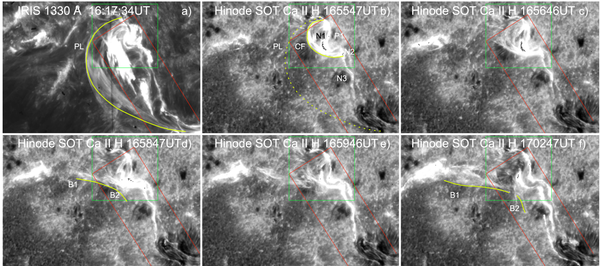
Figure 6. from MULTIWAVELENGTH OBSERVATIONS OF A SLOW-RISE, MULTISTEP X1.6 FLARE AND THE ASSOCIATED ERUPTION null 2015 APJ 812 172 doi:10.1088/0004-637X/812/2/172 https://dx.doi.org/10.1088/0004-637X/812/2/172 © 2015. The American Astronomical Society. All rights reserved.
