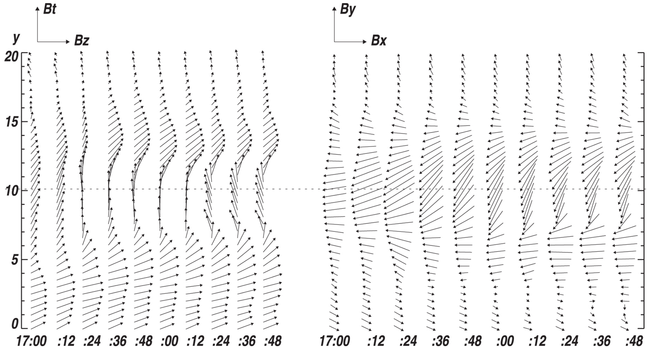
Figure 5. from MULTIWAVELENGTH OBSERVATIONS OF A SLOW-RISE, MULTISTEP X1.6 FLARE AND THE ASSOCIATED ERUPTION null 2015 APJ 812 172 doi:10.1088/0004-637X/812/2/172 https://dx.doi.org/10.1088/0004-637X/812/2/172 © 2015. The American Astronomical Society. All rights reserved.
