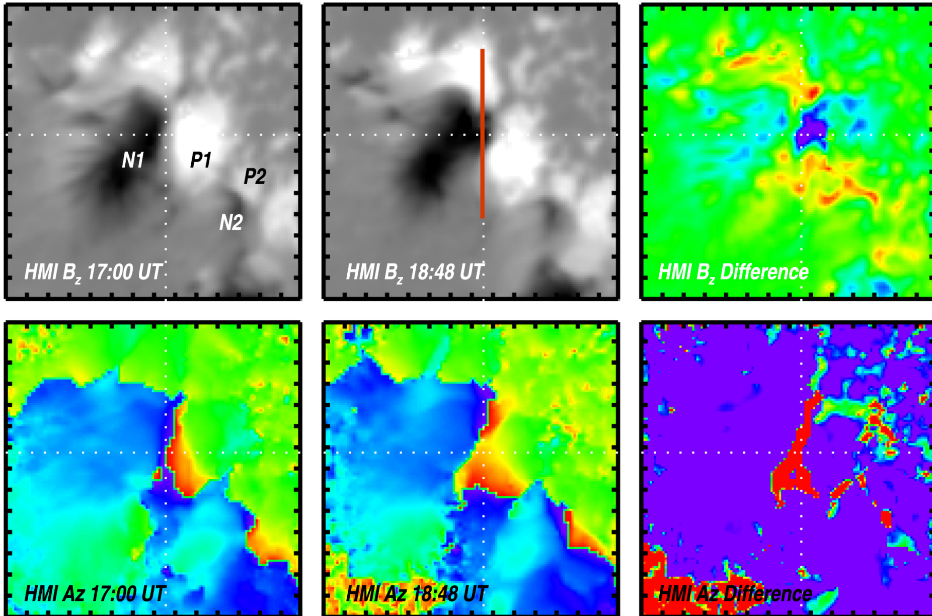
Figure 4. from MULTIWAVELENGTH OBSERVATIONS OF A SLOW-RISE, MULTISTEP X1.6 FLARE AND THE ASSOCIATED ERUPTION null 2015 APJ 812 172 doi:10.1088/0004-637X/812/2/172 https://dx.doi.org/10.1088/0004-637X/812/2/172 © 2015. The American Astronomical Society. All rights reserved.
