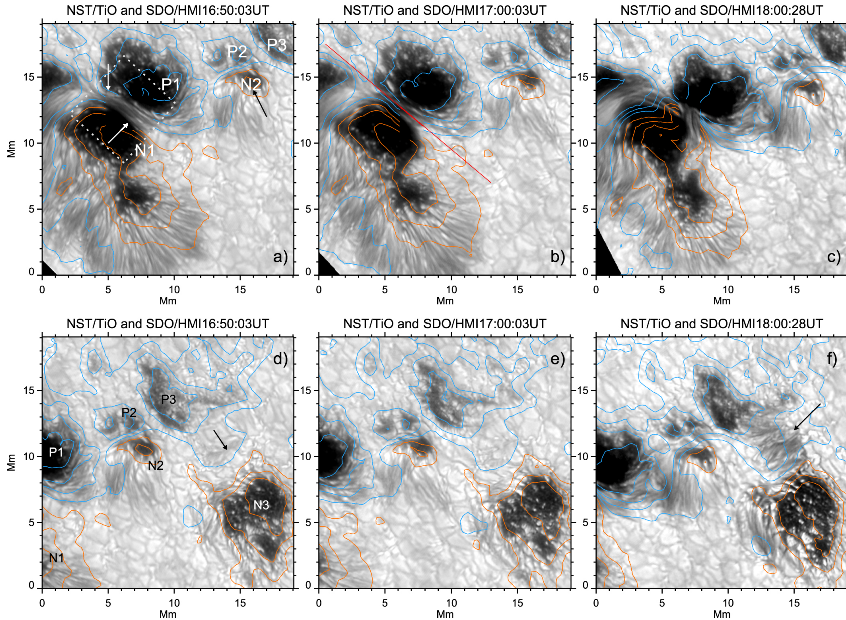
Figure 3. from MULTIWAVELENGTH OBSERVATIONS OF A SLOW-RISE, MULTISTEP X1.6 FLARE AND THE ASSOCIATED ERUPTION null 2015 APJ 812 172 doi:10.1088/0004-637X/812/2/172 https://dx.doi.org/10.1088/0004-637X/812/2/172 © 2015. The American Astronomical Society. All rights reserved.
