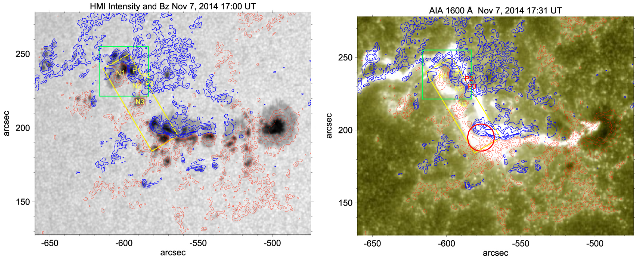
Figure 2. from MULTIWAVELENGTH OBSERVATIONS OF A SLOW-RISE, MULTISTEP X1.6 FLARE AND THE ASSOCIATED ERUPTION null 2015 APJ 812 172 doi:10.1088/0004-637X/812/2/172 https://dx.doi.org/10.1088/0004-637X/812/2/172 © 2015. The American Astronomical Society. All rights reserved.
