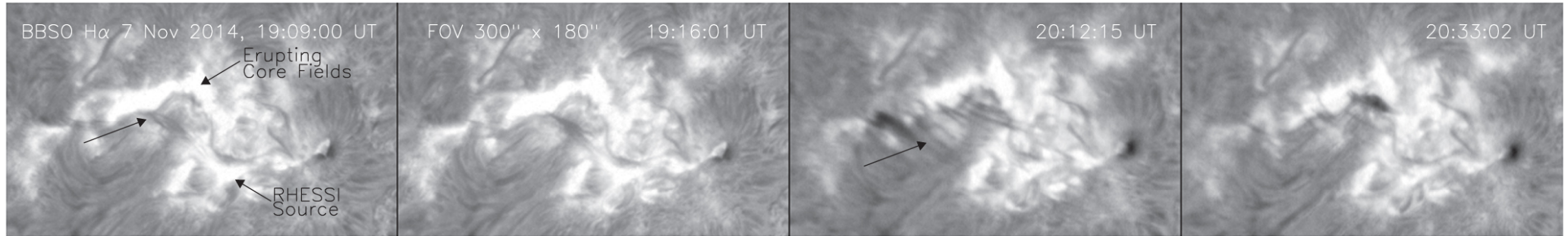
Figure 15. from MULTIWAVELENGTH OBSERVATIONS OF A SLOW-RISE, MULTISTEP X1.6 FLARE AND THE ASSOCIATED ERUPTION null 2015 APJ 812 172 doi:10.1088/0004-637X/812/2/172 https://dx.doi.org/10.1088/0004-637X/812/2/172 © 2015. The American Astronomical Society. All rights reserved.
