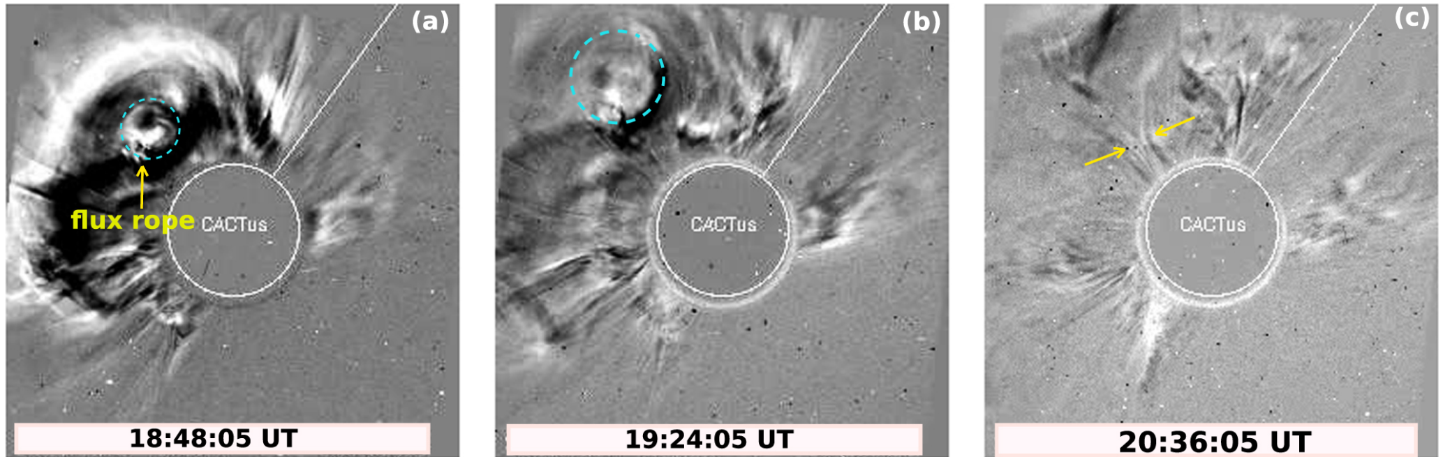
Figure 14. from MULTIWAVELENGTH OBSERVATIONS OF A SLOW-RISE, MULTISTEP X1.6 FLARE AND THE ASSOCIATED ERUPTION null 2015 APJ 812 172 doi:10.1088/0004-637X/812/2/172 https://dx.doi.org/10.1088/0004-637X/812/2/172 © 2015. The American Astronomical Society. All rights reserved.
