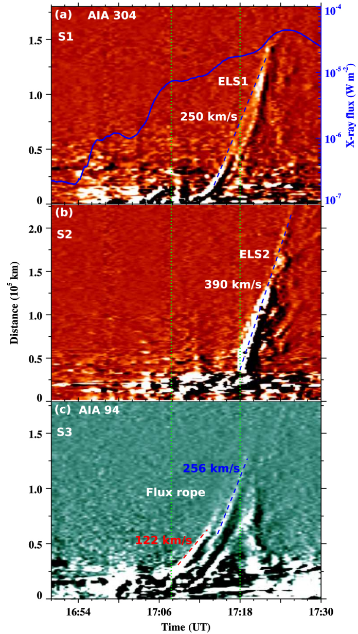
Figure 13. from MULTIWAVELENGTH OBSERVATIONS OF A SLOW-RISE, MULTISTEP X1.6 FLARE AND THE ASSOCIATED ERUPTION null 2015 APJ 812 172 doi:10.1088/0004-637X/812/2/172 https://dx.doi.org/10.1088/0004-637X/812/2/172 © 2015. The American Astronomical Society. All rights reserved.
