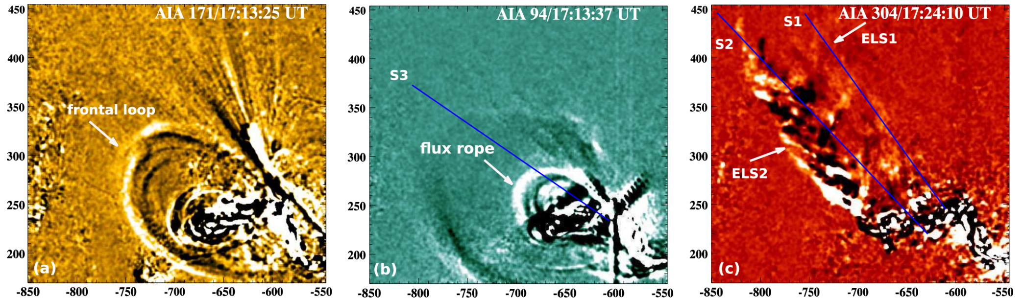
Figure 12. from MULTIWAVELENGTH OBSERVATIONS OF A SLOW-RISE, MULTISTEP X1.6 FLARE AND THE ASSOCIATED ERUPTION null 2015 APJ 812 172 doi:10.1088/0004-637X/812/2/172 https://dx.doi.org/10.1088/0004-637X/812/2/172 © 2015. The American Astronomical Society. All rights reserved.
