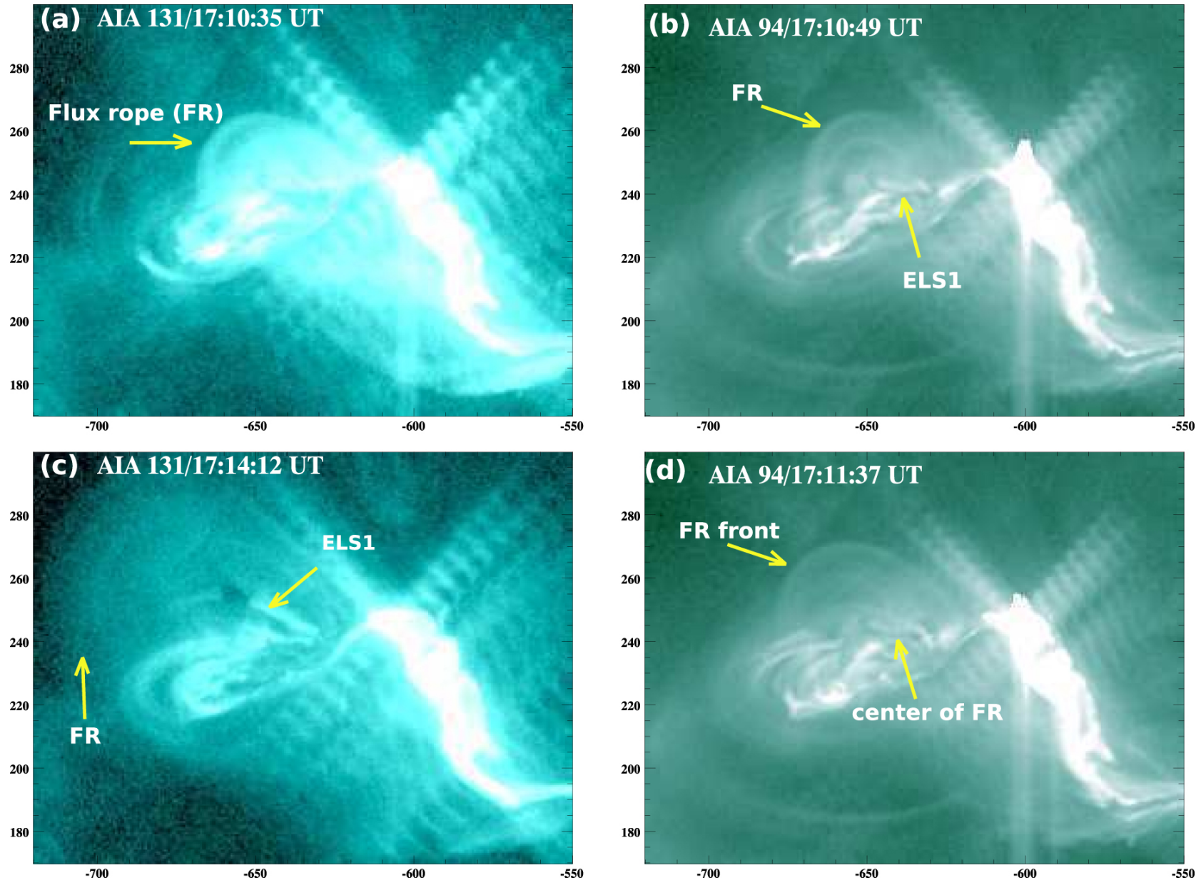
Figure 11. from MULTIWAVELENGTH OBSERVATIONS OF A SLOW-RISE, MULTISTEP X1.6 FLARE AND THE ASSOCIATED ERUPTION null 2015 APJ 812 172 doi:10.1088/0004-637X/812/2/172 https://dx.doi.org/10.1088/0004-637X/812/2/172 © 2015. The American Astronomical Society. All rights reserved.
