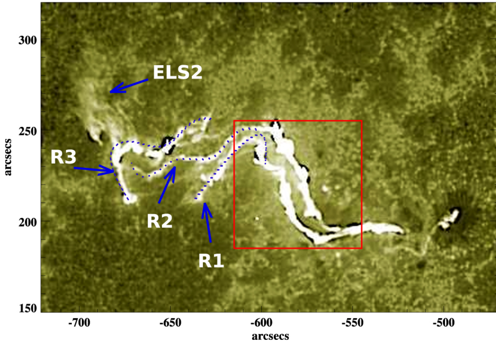
Figure 10. from MULTIWAVELENGTH OBSERVATIONS OF A SLOW-RISE, MULTISTEP X1.6 FLARE AND THE ASSOCIATED ERUPTION null 2015 APJ 812 172 doi:10.1088/0004-637X/812/2/172 https://dx.doi.org/10.1088/0004-637X/812/2/172 © 2015. The American Astronomical Society. All rights reserved.
