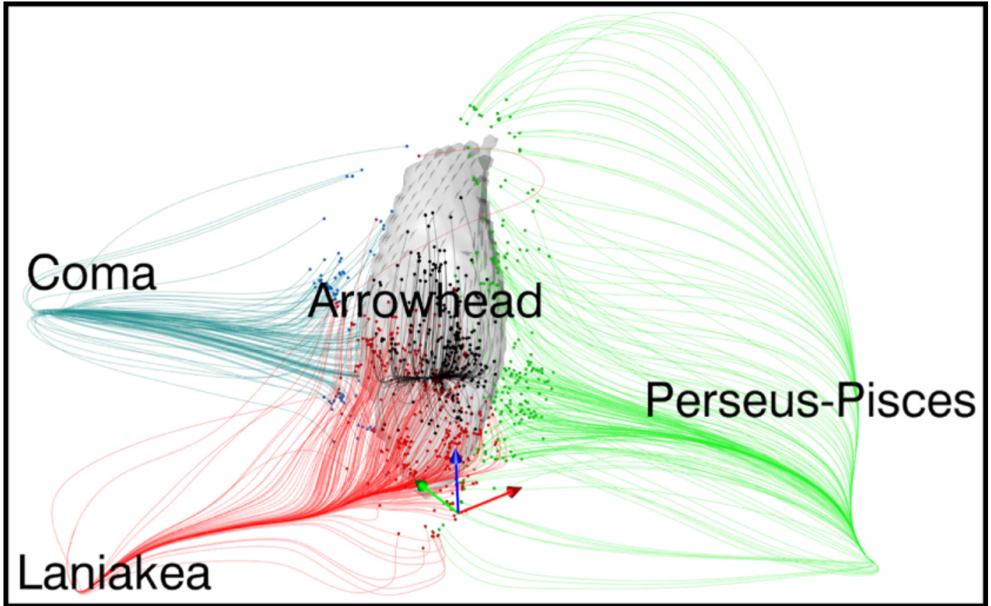
Figure 6. from THE ARROWHEAD MINI-SUPERCLUSTER OF GALAXIES null 2015 APJ 812 17 doi:10.1088/0004-637X/812/1/17 https://dx.doi.org/10.1088/0004-637X/812/1/17 © 2015. The American Astronomical Society. All rights reserved.
