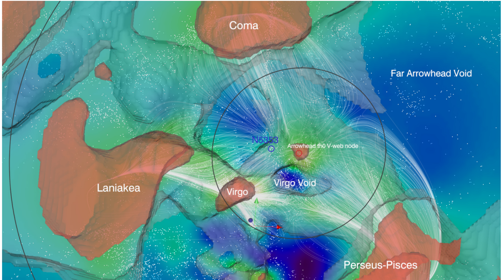
Figure 5. from THE ARROWHEAD MINI-SUPERCLUSTER OF GALAXIES null 2015 APJ 812 17 doi:10.1088/0004-637X/812/1/17 https://dx.doi.org/10.1088/0004-637X/812/1/17 © 2015. The American Astronomical Society. All rights reserved.
