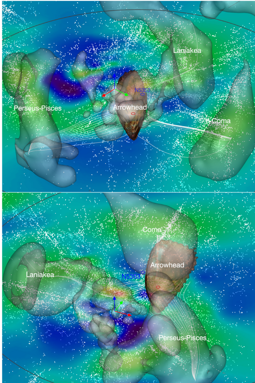
Figure 4. from THE ARROWHEAD MINI-SUPERCLUSTER OF GALAXIES null 2015 APJ 812 17 doi:10.1088/0004-637X/812/1/17 https://dx.doi.org/10.1088/0004-637X/812/1/17 © 2015. The American Astronomical Society. All rights reserved.
