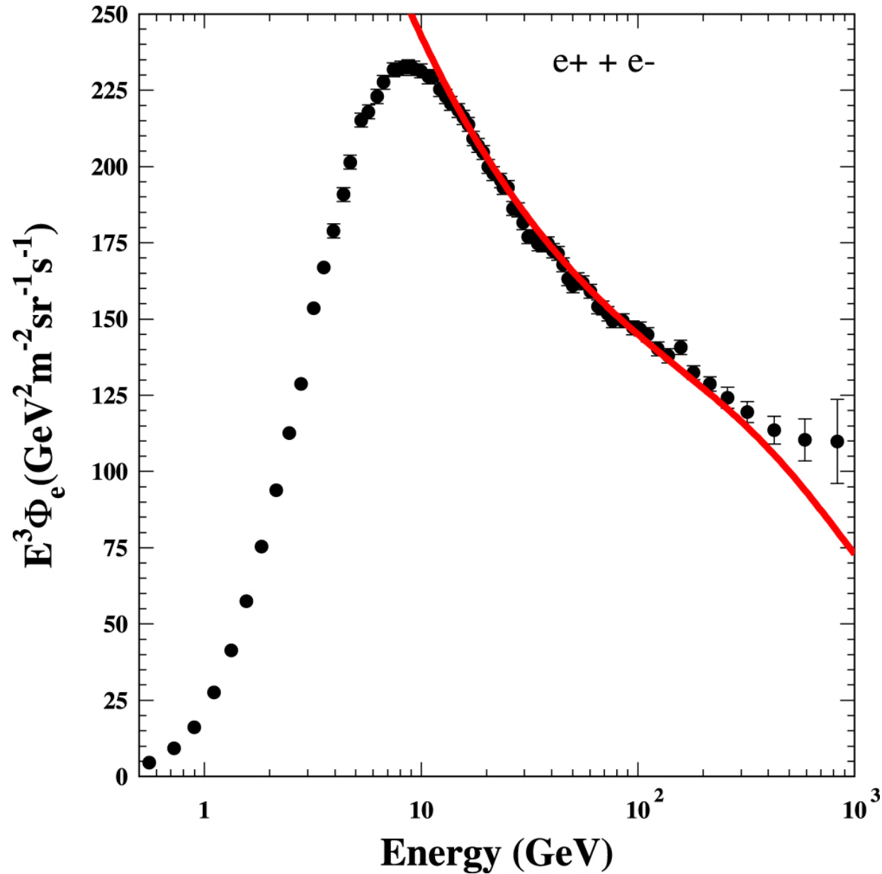
Figure 8. from ORIGIN OF THE COSMIC RAY POSITRONS OBSERVED NEAR EARTH: MESON DECAY OR DARK MATTER DECAY? null 2015 APJ 812 38 doi:10.1088/0004-637X/812/1/38 https://dx.doi.org/10.1088/0004-637X/812/1/38 © 2015. The American Astronomical Society. All rights reserved.
