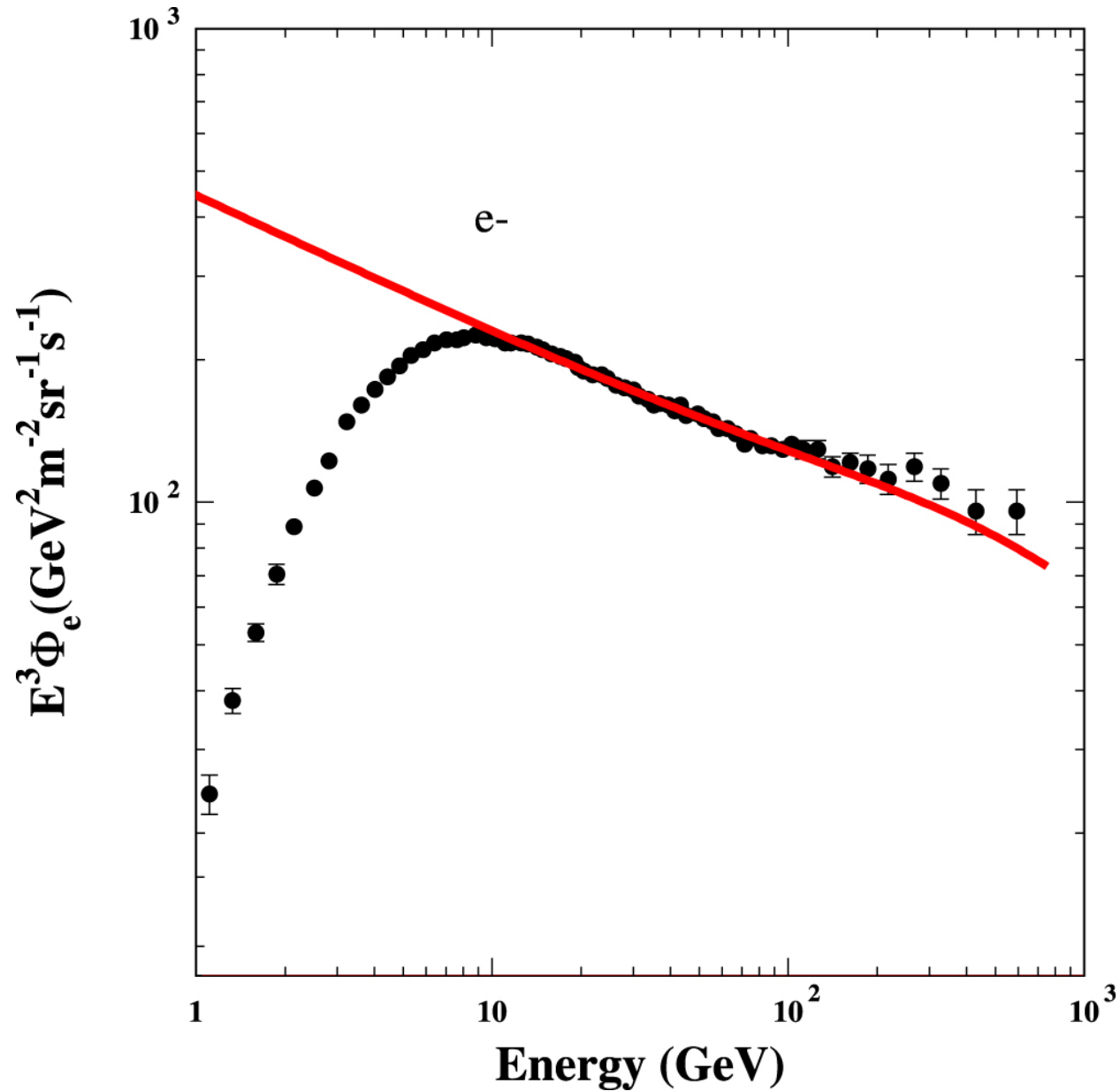
Figure 7. from ORIGIN OF THE COSMIC RAY POSITRONS OBSERVED NEAR EARTH: MESON DECAY OR DARK MATTER DECAY? null 2015 APJ 812 38 doi:10.1088/0004-637X/812/1/38 https://dx.doi.org/10.1088/0004-637X/812/1/38 © 2015. The American Astronomical Society. All rights reserved.
