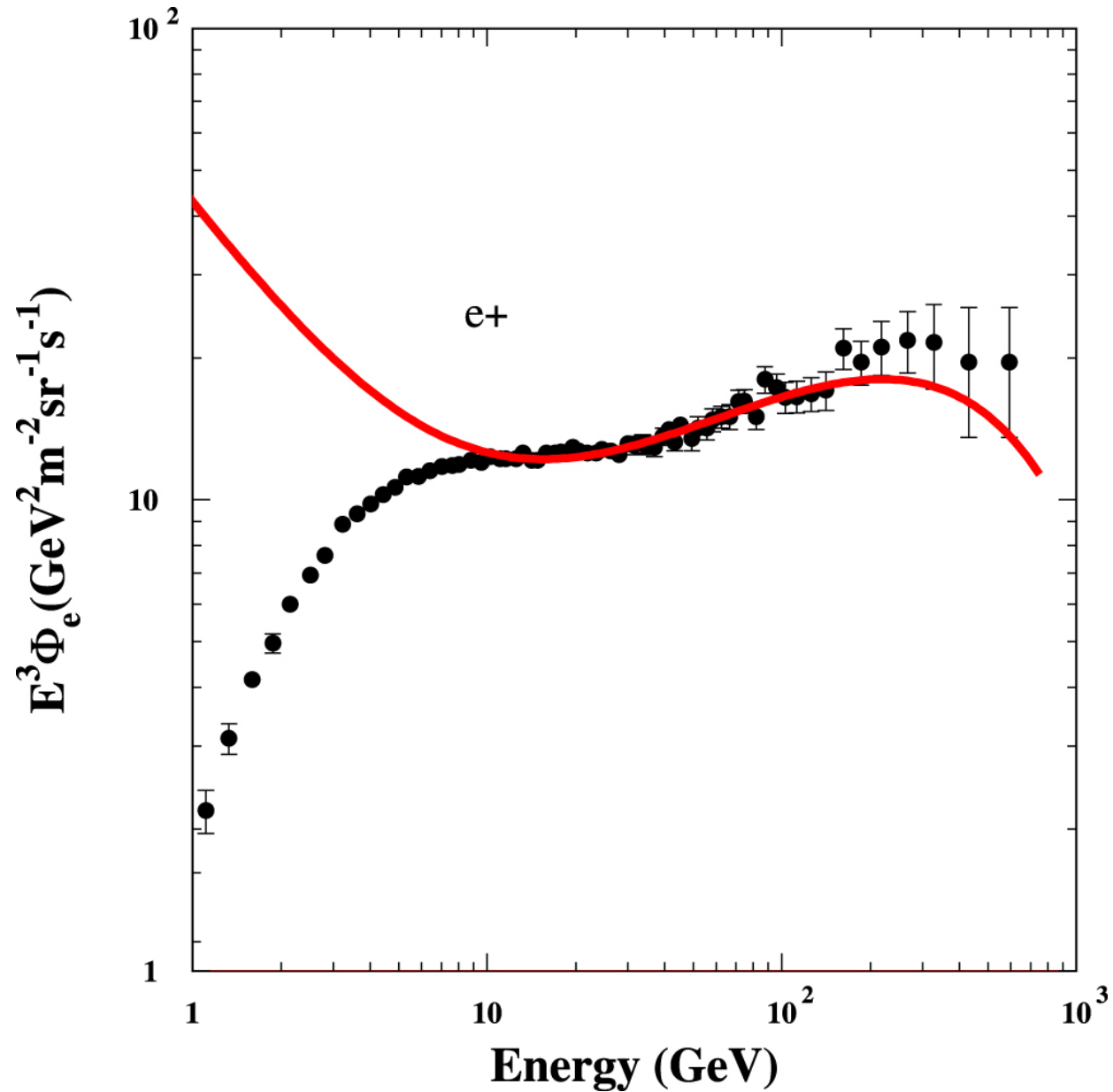
Figure 6. from ORIGIN OF THE COSMIC RAY POSITRONS OBSERVED NEAR EARTH: MESON DECAY OR DARK MATTER DECAY? null 2015 APJ 812 38 doi:10.1088/0004-637X/812/1/38 https://dx.doi.org/10.1088/0004-637X/812/1/38 © 2015. The American Astronomical Society. All rights reserved.
