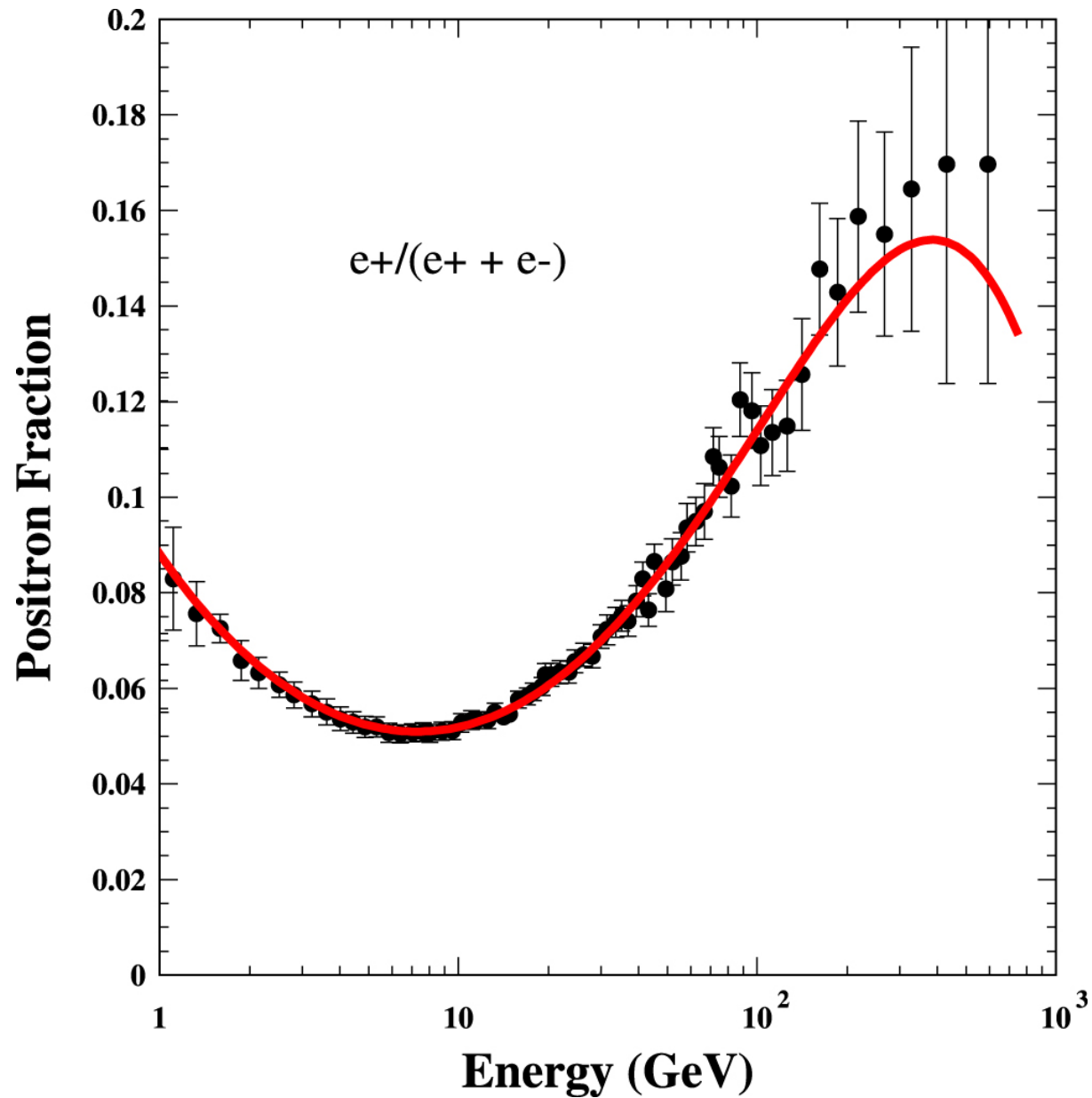
Figure 5. from ORIGIN OF THE COSMIC RAY POSITRONS OBSERVED NEAR EARTH: MESON DECAY OR DARK MATTER DECAY? null 2015 APJ 812 38 doi:10.1088/0004-637X/812/1/38 https://dx.doi.org/10.1088/0004-637X/812/1/38 © 2015. The American Astronomical Society. All rights reserved.
