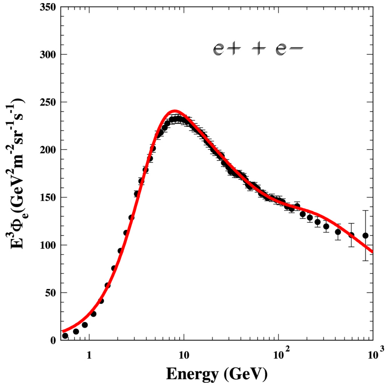
Figure 4. from ORIGIN OF THE COSMIC RAY POSITRONS OBSERVED NEAR EARTH: MESON DECAY OR DARK MATTER DECAY? null 2015 APJ 812 38 doi:10.1088/0004-637X/812/1/38 https://dx.doi.org/10.1088/0004-637X/812/1/38 © 2015. The American Astronomical Society. All rights reserved.
