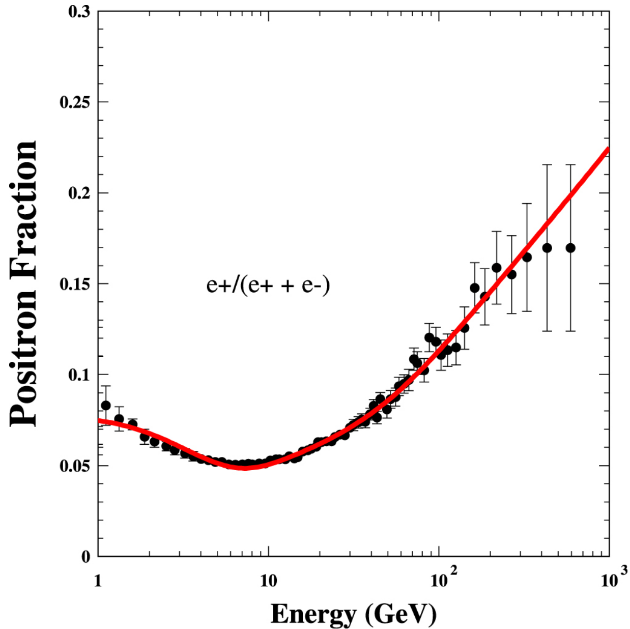
Figure 3. from ORIGIN OF THE COSMIC RAY POSITRONS OBSERVED NEAR EARTH: MESON DECAY OR DARK MATTER DECAY? null 2015 APJ 812 38 doi:10.1088/0004-637X/812/1/38 https://dx.doi.org/10.1088/0004-637X/812/1/38 © 2015. The American Astronomical Society. All rights reserved.
