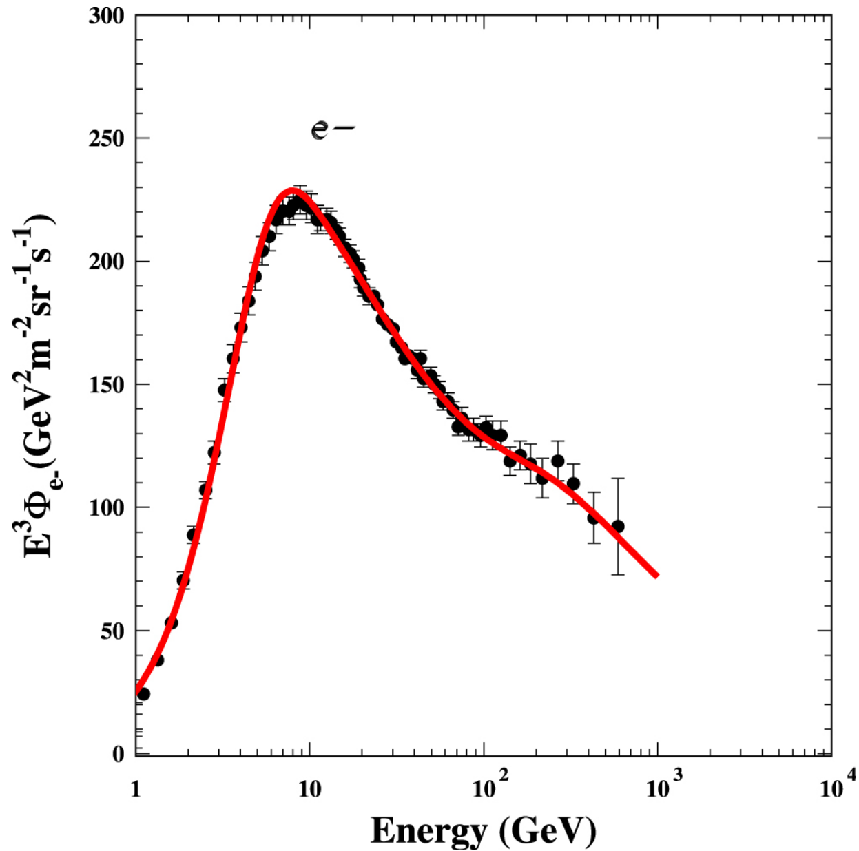
Figure 2. from ORIGIN OF THE COSMIC RAY POSITRONS OBSERVED NEAR EARTH: MESON DECAY OR DARK MATTER DECAY? null 2015 APJ 812 38 doi:10.1088/0004-637X/812/1/38 https://dx.doi.org/10.1088/0004-637X/812/1/38 © 2015. The American Astronomical Society. All rights reserved.
