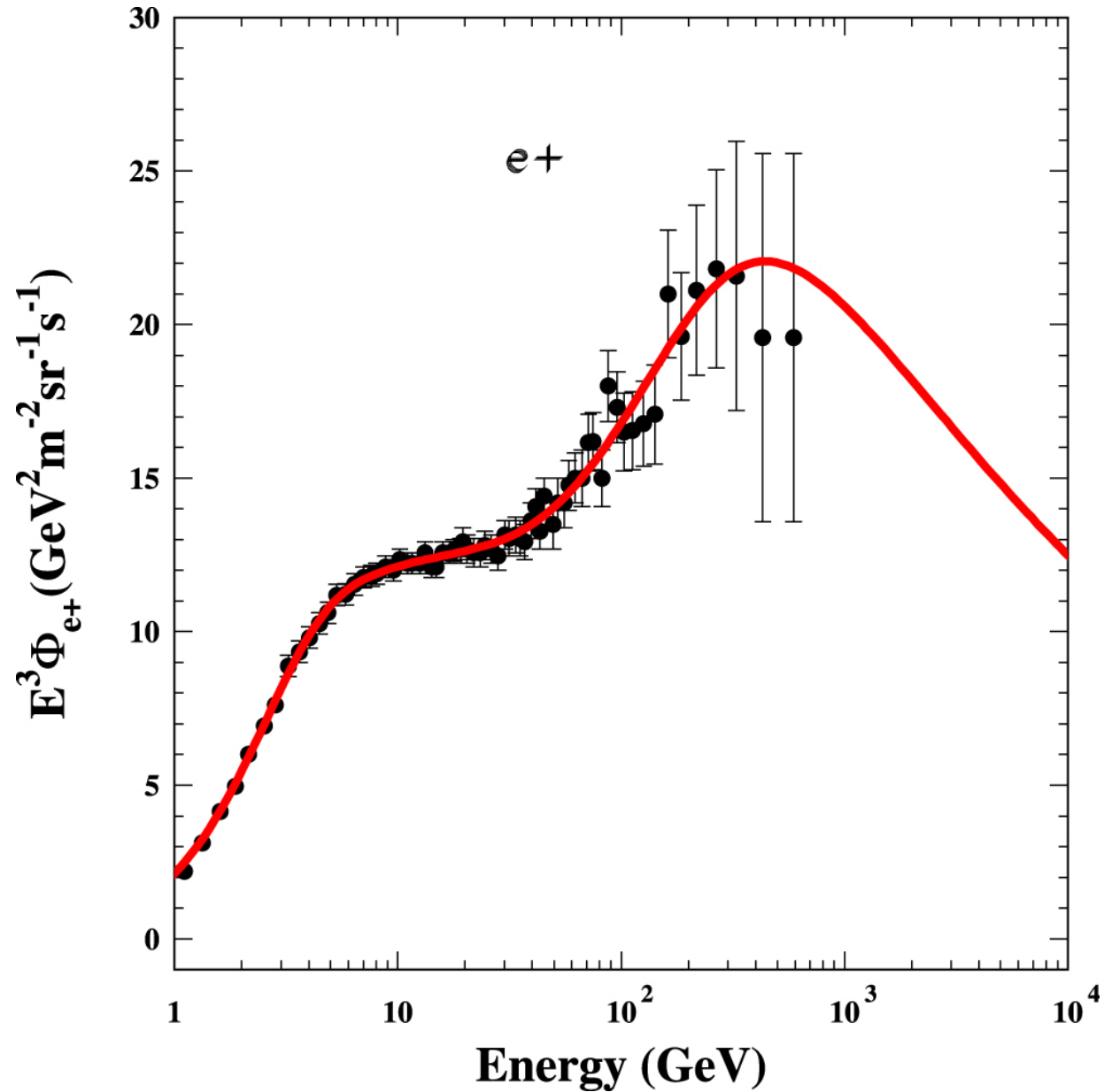
Figure 1. from ORIGIN OF THE COSMIC RAY POSITRONS OBSERVED NEAR EARTH: MESON DECAY OR DARK MATTER DECAY? null 2015 APJ 812 38 doi:10.1088/0004-637X/812/1/38 https://dx.doi.org/10.1088/0004-637X/812/1/38 © 2015. The American Astronomical Society. All rights reserved.
