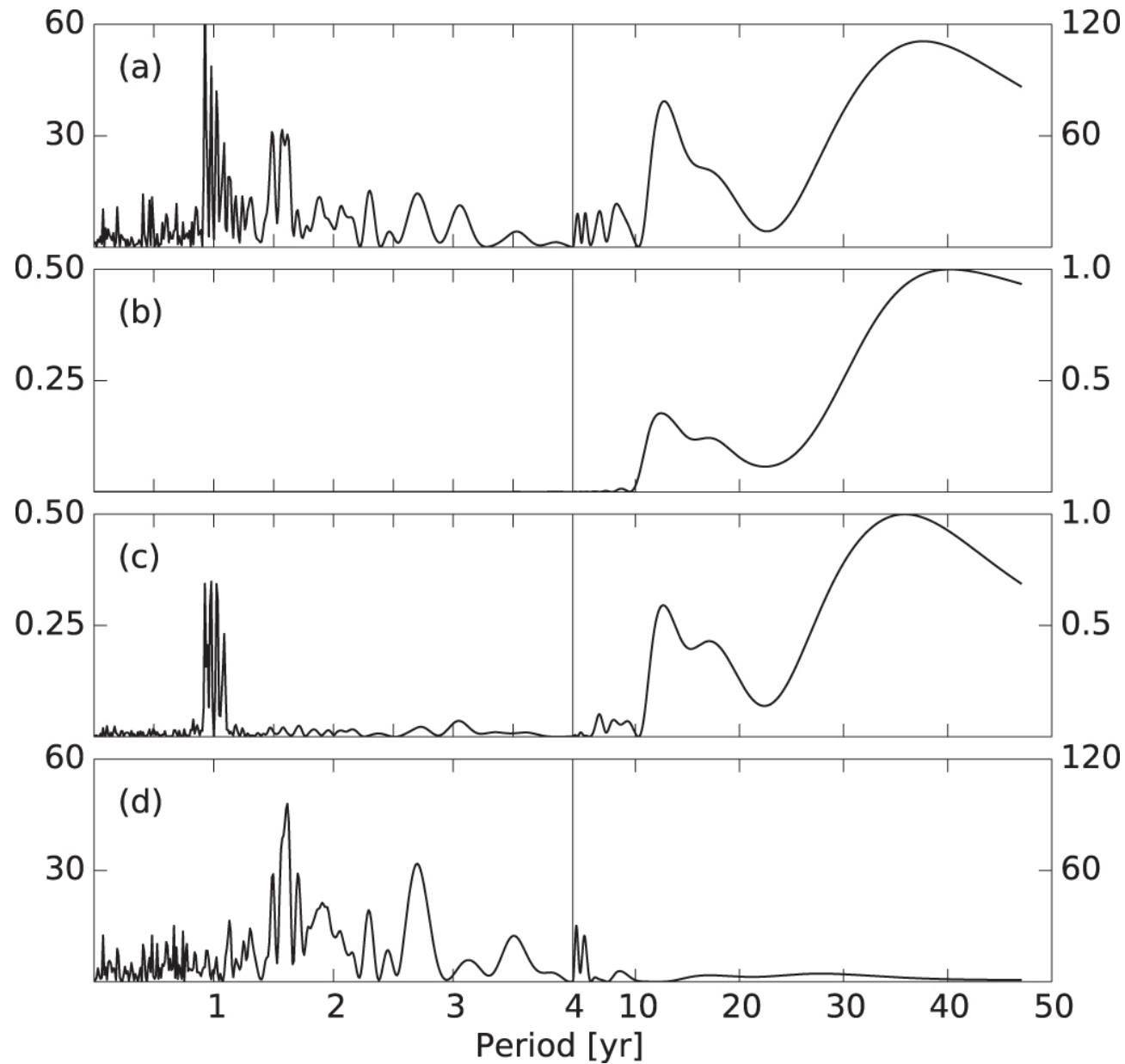
Figure 4. from SUN-LIKE MAGNETIC CYCLES IN THE RAPIDLY ROTATING YOUNG SOLAR ANALOG HD 30495 null 2015 APJ 812 12 doi:10.1088/0004-637X/812/1/12 https://dx.doi.org/10.1088/0004-637X/812/1/12
