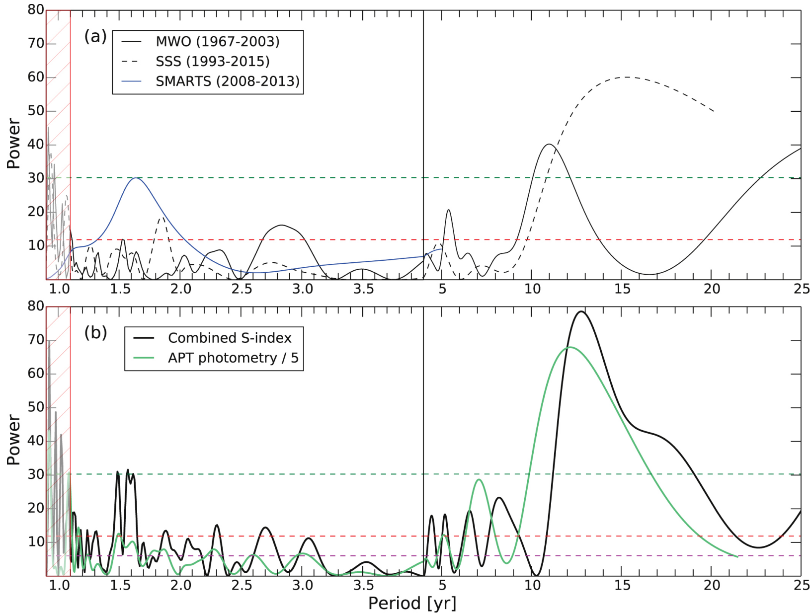
Figure 3. from SUN-LIKE MAGNETIC CYCLES IN THE RAPIDLY ROTATING YOUNG SOLAR ANALOG HD 30495 null 2015 APJ 812 12 doi:10.1088/0004-637X/812/1/12 https://dx.doi.org/10.1088/0004-637X/812/1/12
