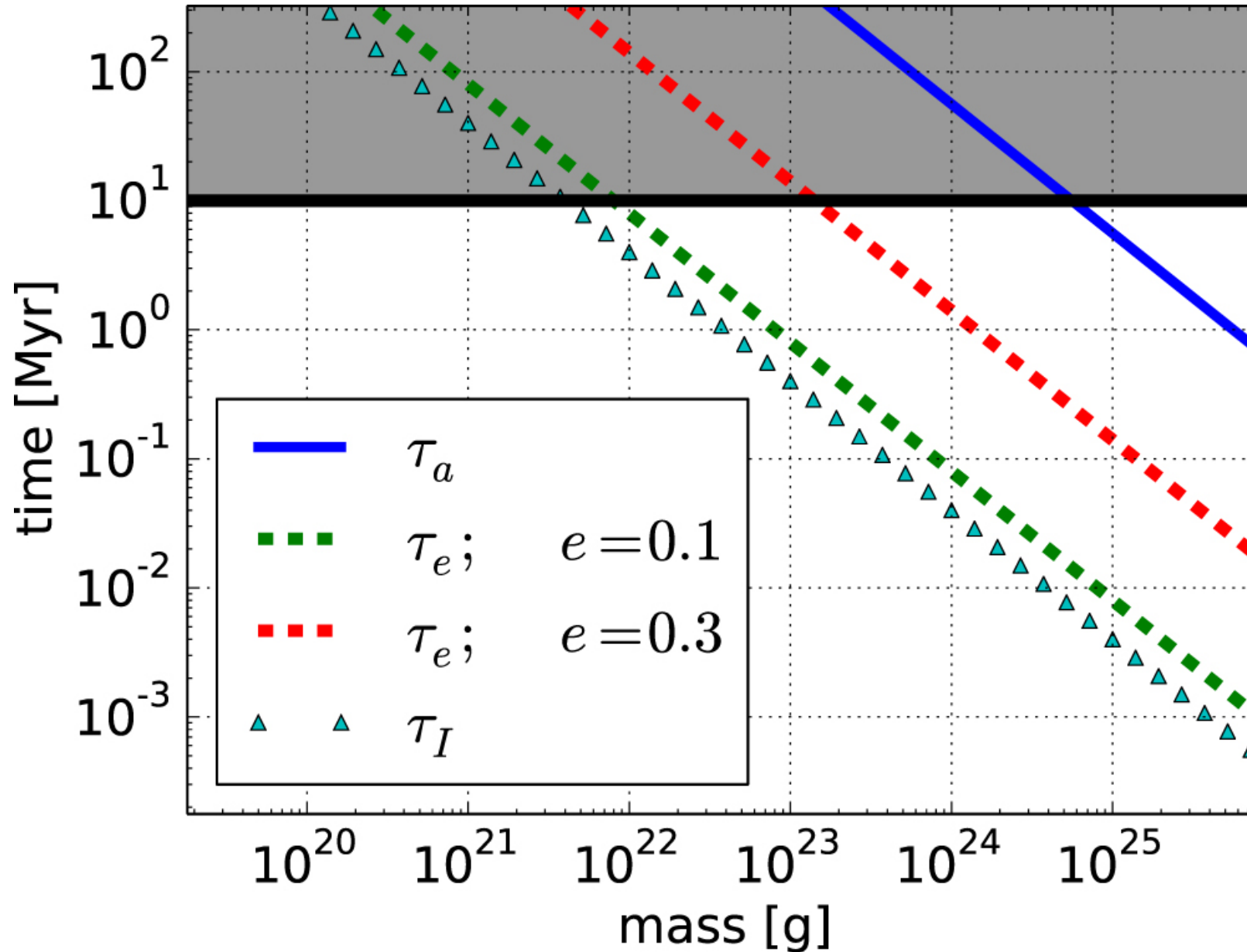
Figure 8. from APPLICATION OF GAS DYNAMICAL FRICTION FOR PLANETESIMALS. I. EVOLUTION OF SINGLE PLANETESIMALS null 2015 APJ 811 54 doi:10.1088/0004-637X/811/1/54 https://dx.doi.org/10.1088/0004-637X/811/1/54 © 2015. The American Astronomical Society. All rights reserved.
