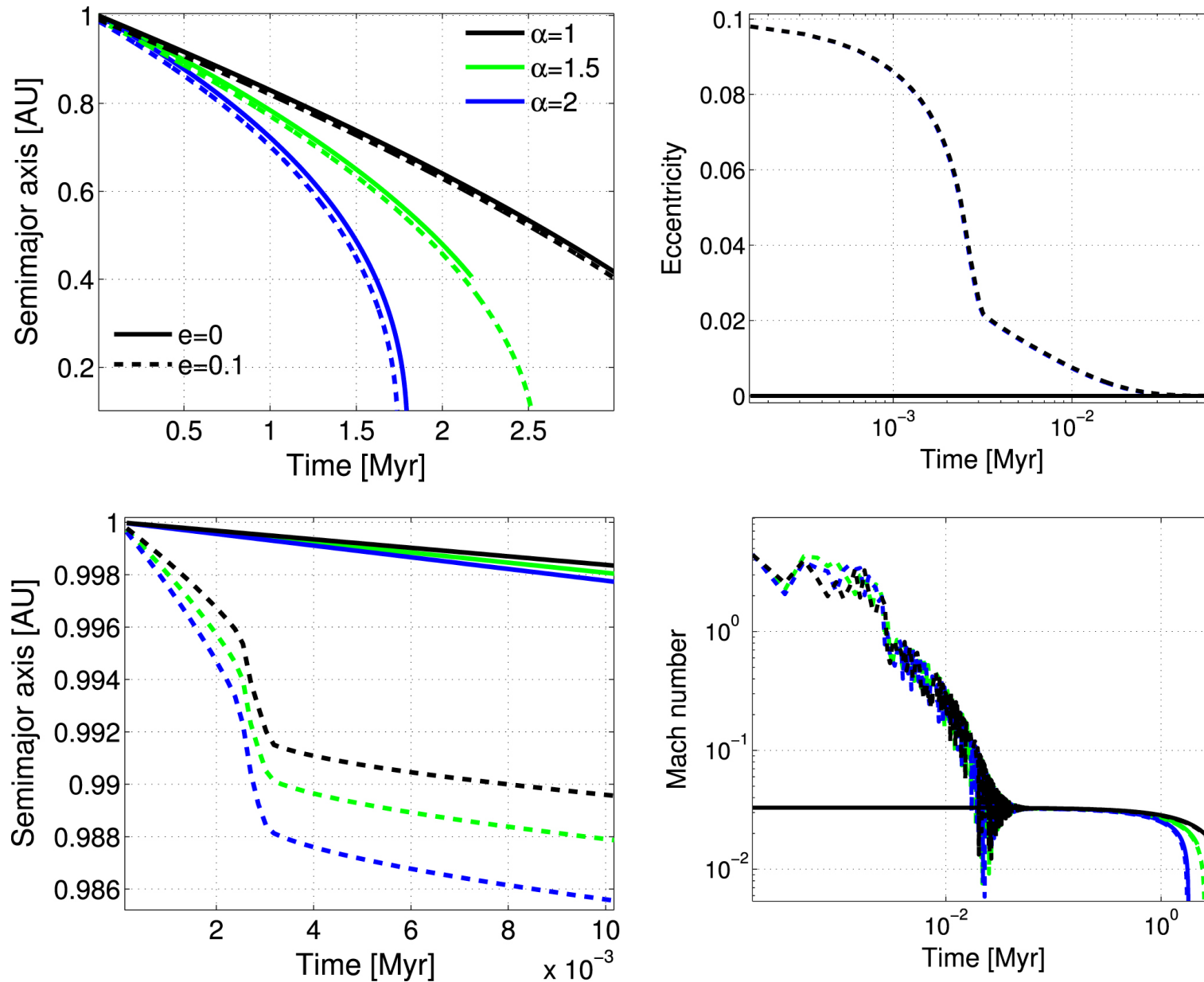
Figure 6. from APPLICATION OF GAS DYNAMICAL FRICTION FOR PLANETESIMALS. I. EVOLUTION OF SINGLE PLANETESIMALS null 2015 APJ 811 54 doi:10.1088/0004-637X/811/1/54 https://dx.doi.org/10.1088/0004-637X/811/1/54 © 2015. The American Astronomical Society. All rights reserved.
