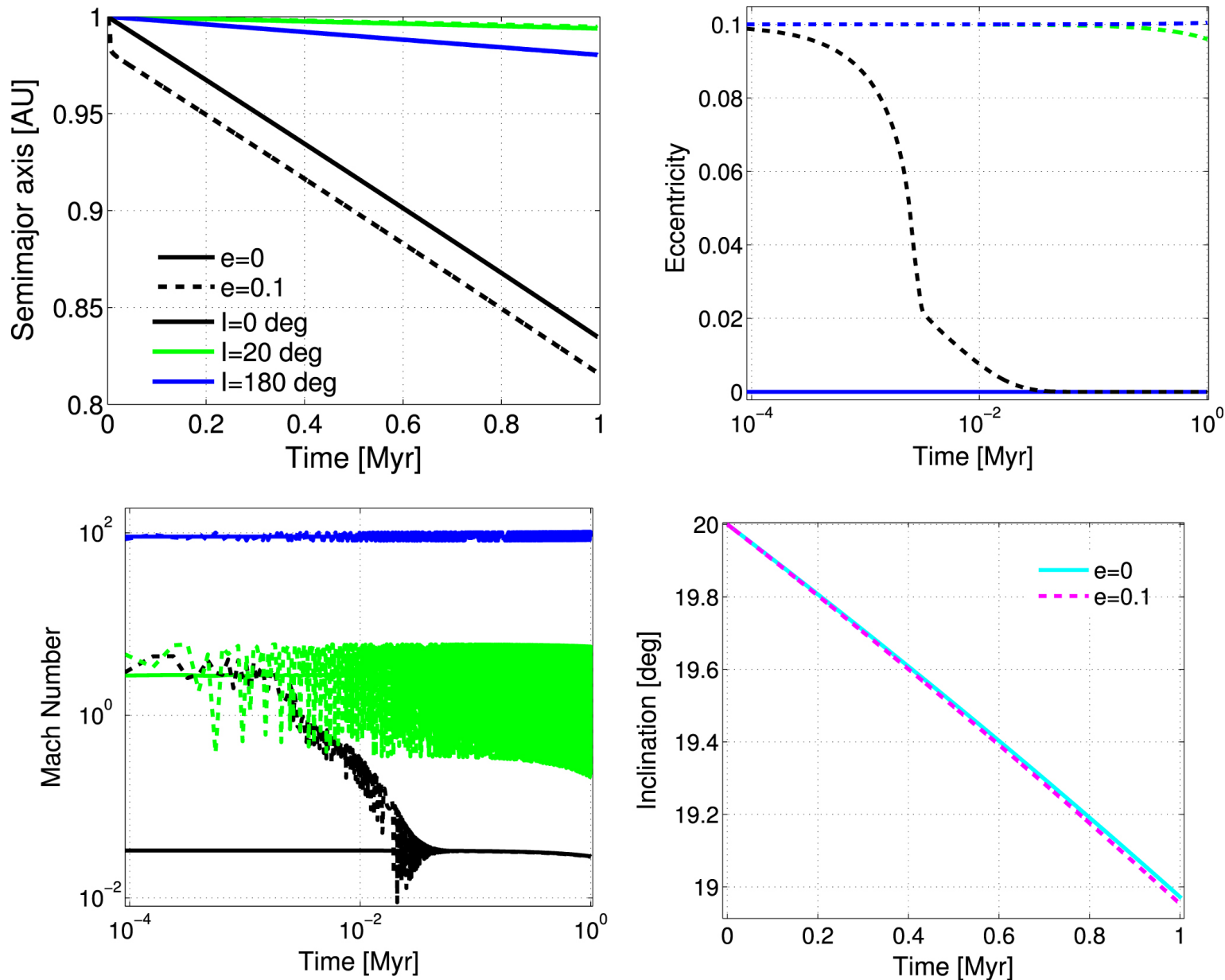
Figure 5. from APPLICATION OF GAS DYNAMICAL FRICTION FOR PLANETESIMALS. I. EVOLUTION OF SINGLE PLANETESIMALS null 2015 APJ 811 54 doi:10.1088/0004-637X/811/1/54 https://dx.doi.org/10.1088/0004-637X/811/1/54 © 2015. The American Astronomical Society. All rights reserved.
