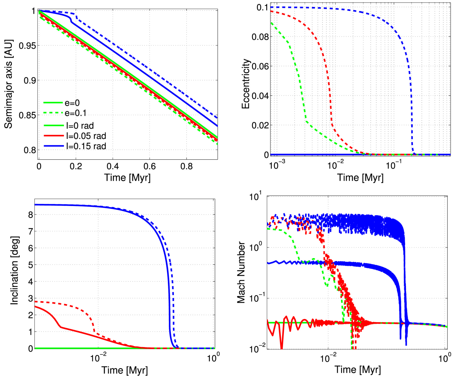
Figure 4. from APPLICATION OF GAS DYNAMICAL FRICTION FOR PLANETESIMALS. I. EVOLUTION OF SINGLE PLANETESIMALS null 2015 APJ 811 54 doi:10.1088/0004-637X/811/1/54 https://dx.doi.org/10.1088/0004-637X/811/1/54 © 2015. The American Astronomical Society. All rights reserved.
